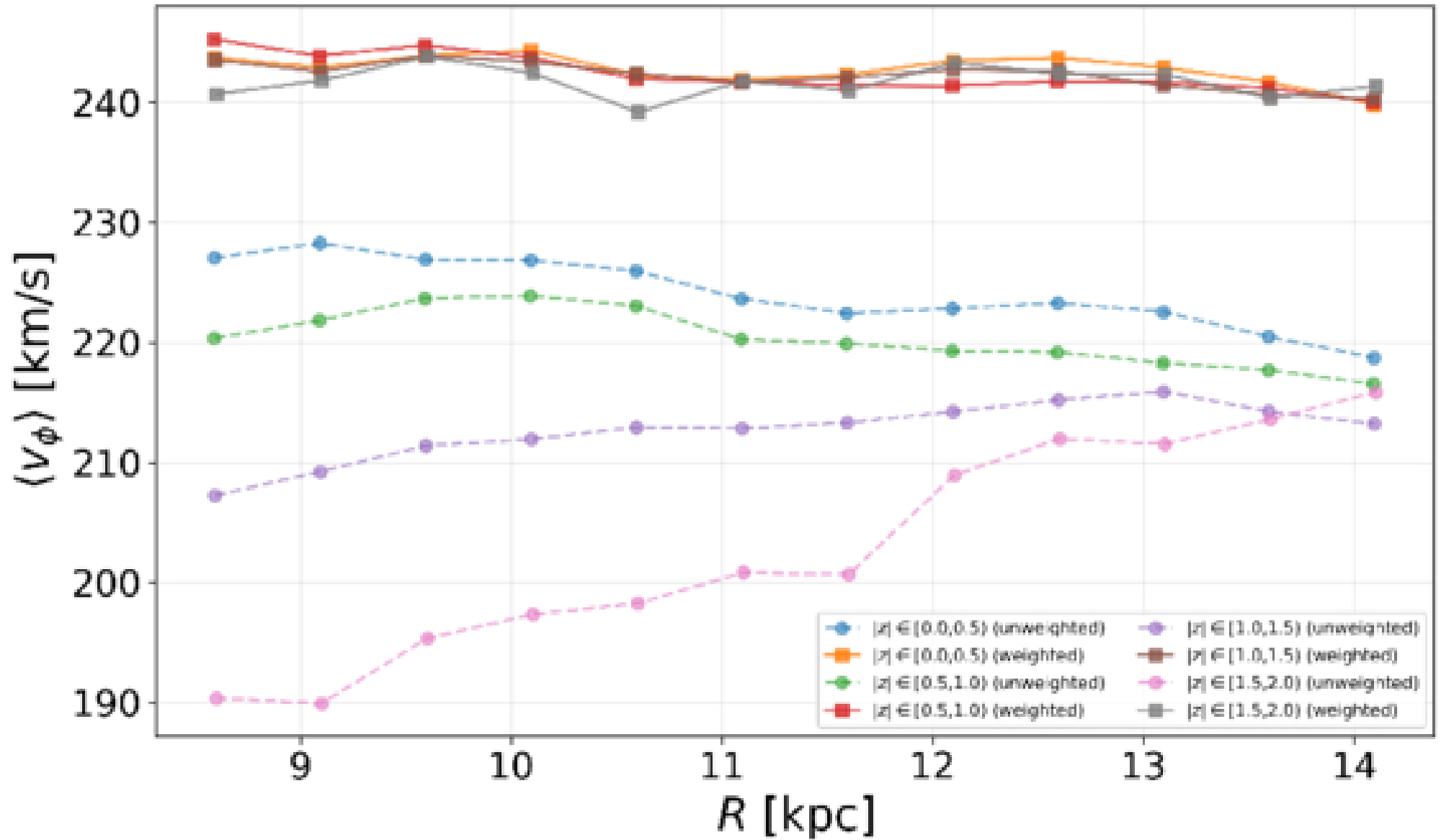
Figure 2. from Francesco Sylos Labini and Roberto Capuzzo-Dolcetta 2026 Astrophys. J. 1005 doi:10.3847/1538-4357/ae7be7 https://dx.doi.org/10.3847/1538-4357/ae7be7 © 2026. The Author(s). Published by the American Astronomical Society.
