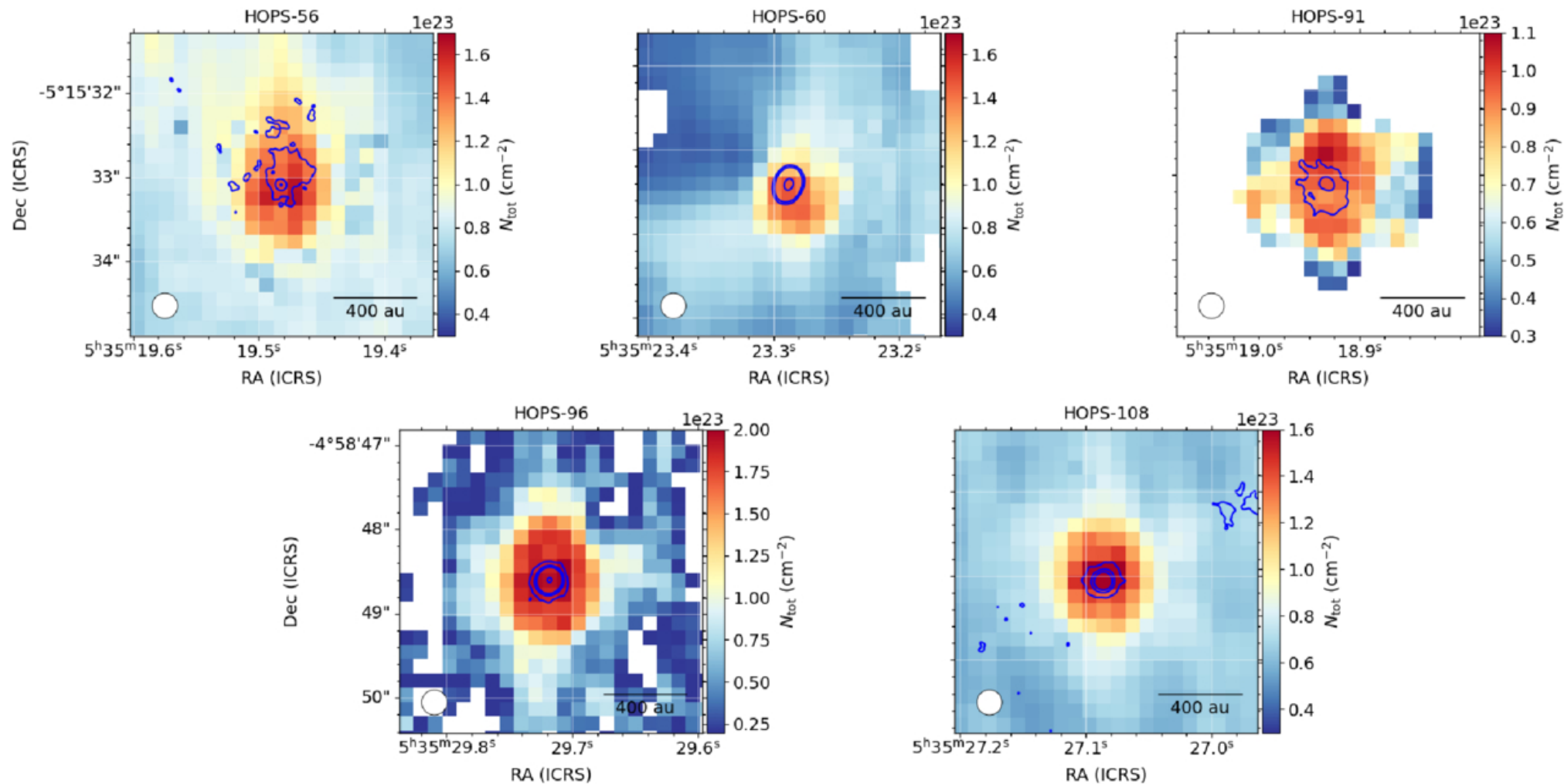
Figure 8. from Igor Petrashkevich et al 2026 Astrophys. J. 1006 doi:10.3847/1538-4357/ae7b20 https://dx.doi.org/10.3847/1538-4357/ae7b20 © 2026. The Author(s). Published by the American Astronomical Society.
