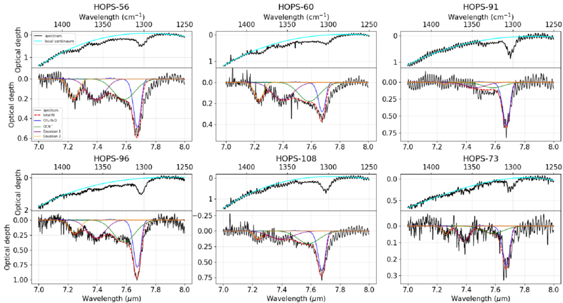
Figure 7. from Igor Petrashkevich et al 2026 Astrophys. J. 1006 doi:10.3847/1538-4357/ae7b20 https://dx.doi.org/10.3847/1538-4357/ae7b20 © 2026. The Author(s). Published by the American Astronomical Society.
