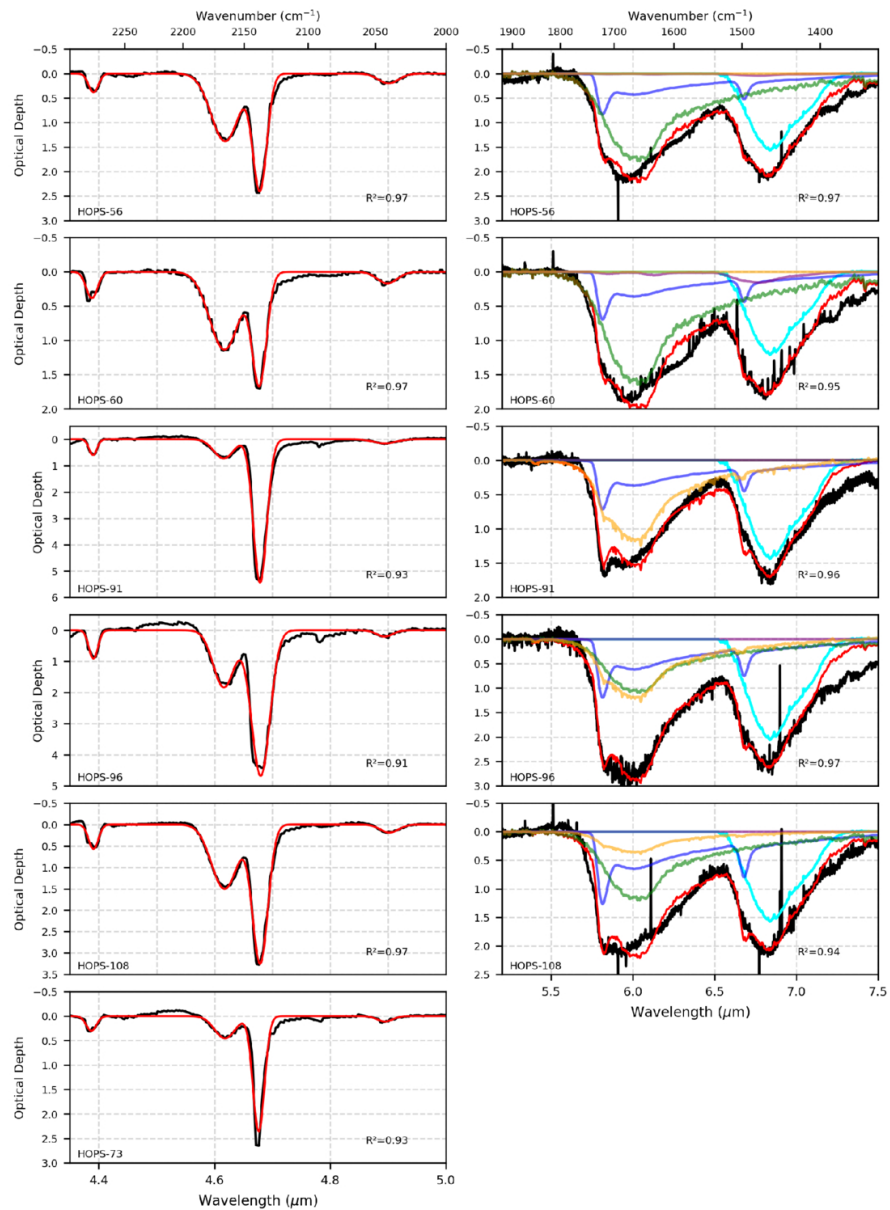
Figure 6. from Igor Petrashkevich et al 2026 Astrophys. J. 1006 doi:10.3847/1538-4357/ae7b20 https://dx.doi.org/10.3847/1538-4357/ae7b20 © 2026. The Author(s). Published by the American Astronomical Society.
