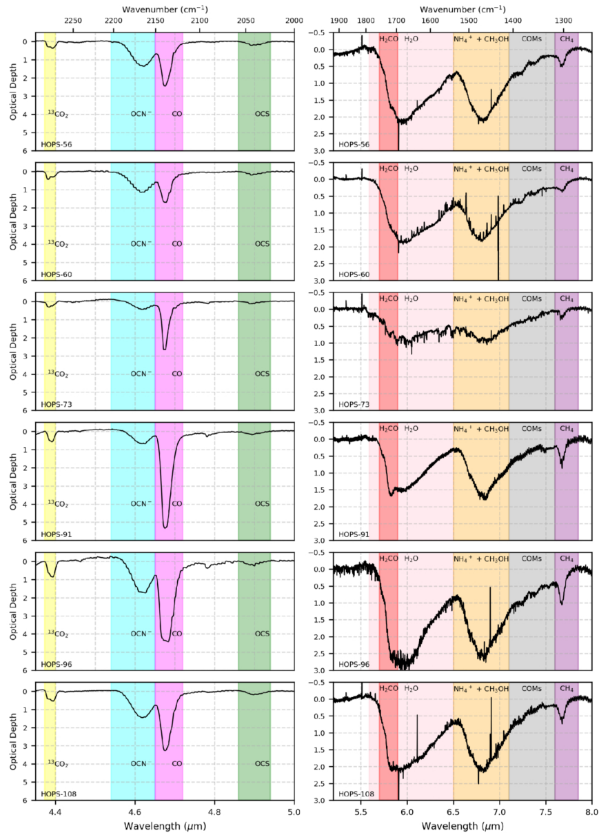
Figure 4. from Igor Petrashkevich et al 2026 Astrophys. J. 1006 doi:10.3847/1538-4357/ae7b20 https://dx.doi.org/10.3847/1538-4357/ae7b20 © 2026. The Author(s). Published by the American Astronomical Society.
