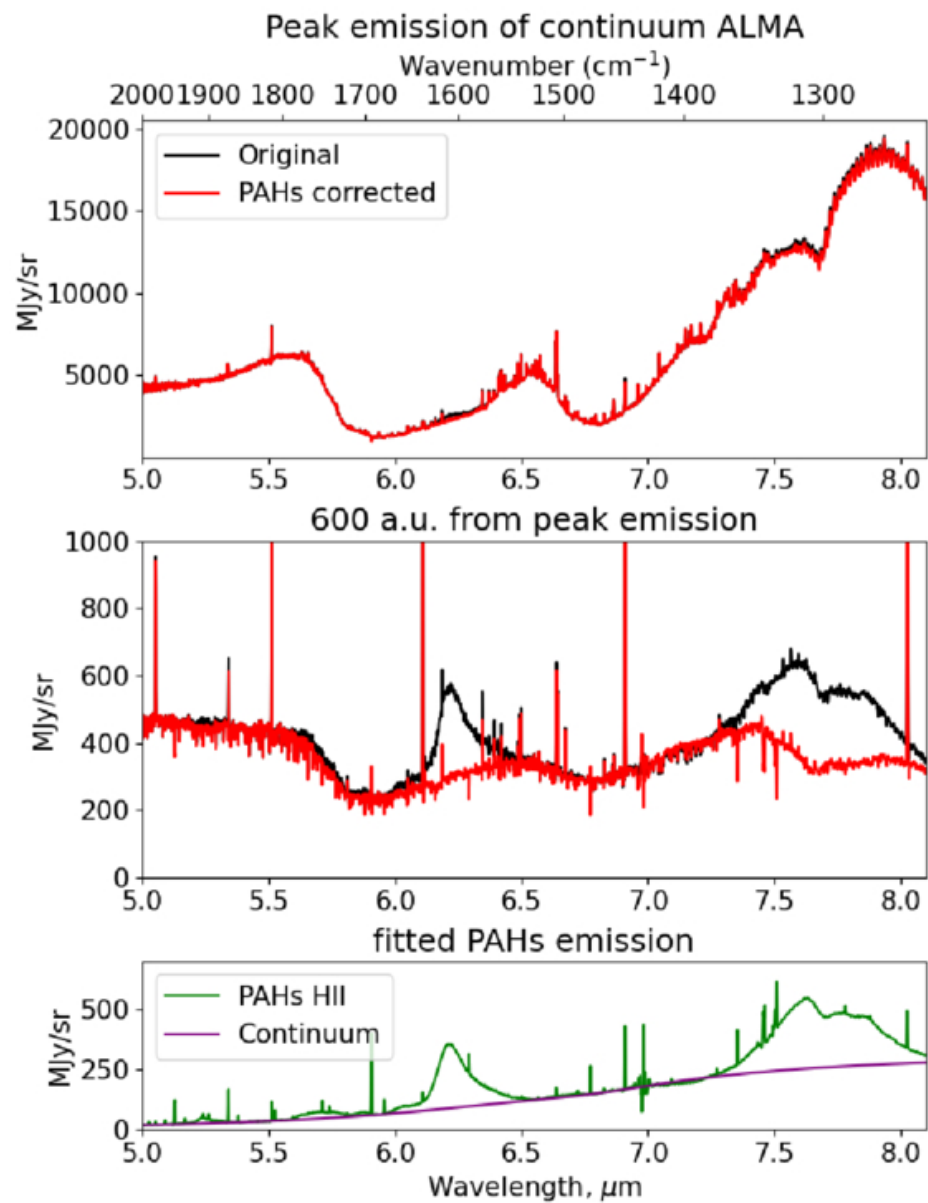
Figure 3. from Igor Petrashkevich et al 2026 Astrophys. J. 1006 doi:10.3847/1538-4357/ae7b20 https://dx.doi.org/10.3847/1538-4357/ae7b20 © 2026. The Author(s). Published by the American Astronomical Society.
