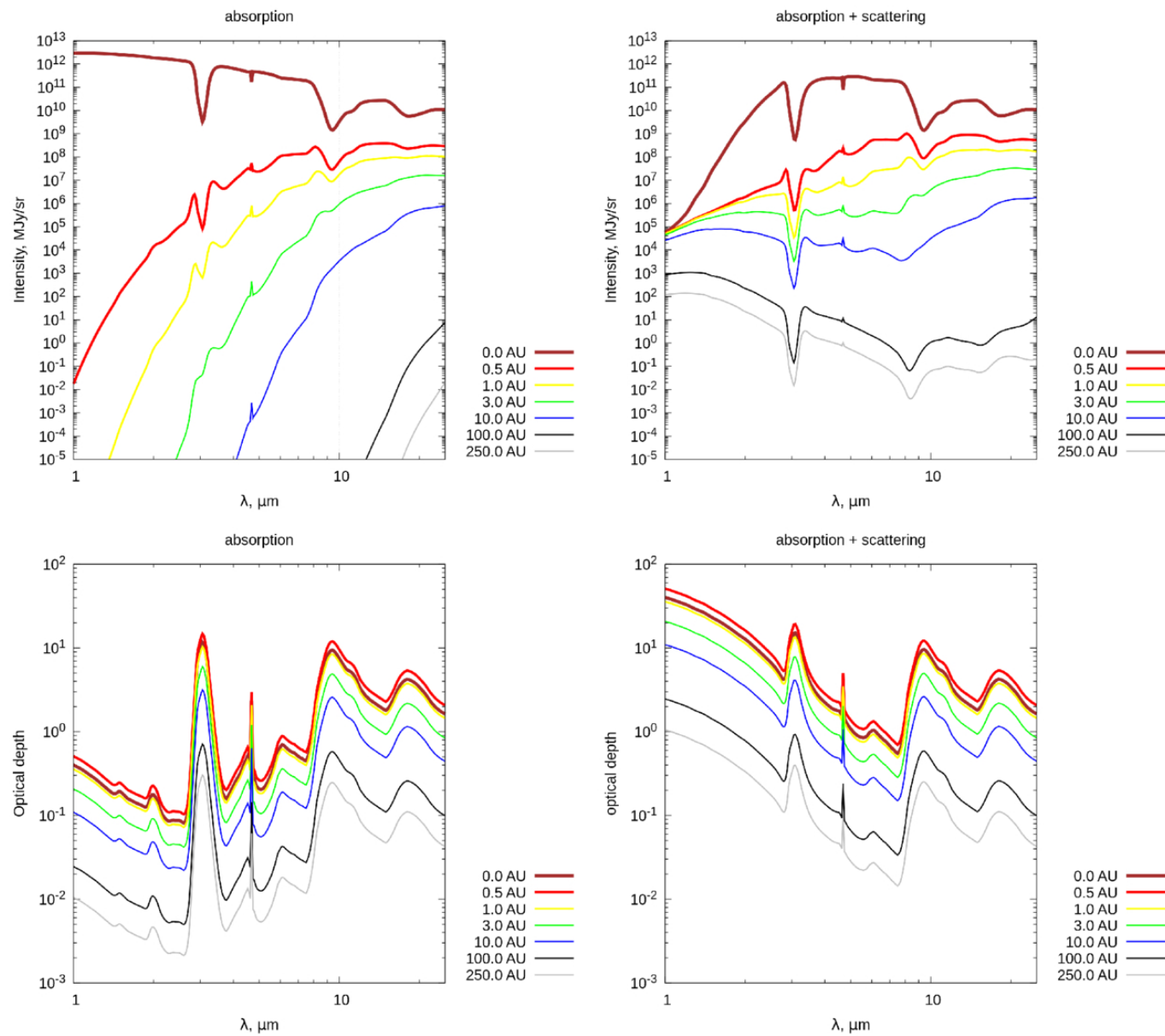
Figure 13. from Igor Petrashkevich et al 2026 Astrophys. J. 1006 doi:10.3847/1538-4357/ae7b20 https://dx.doi.org/10.3847/1538-4357/ae7b20 © 2026. The Author(s). Published by the American Astronomical Society.
