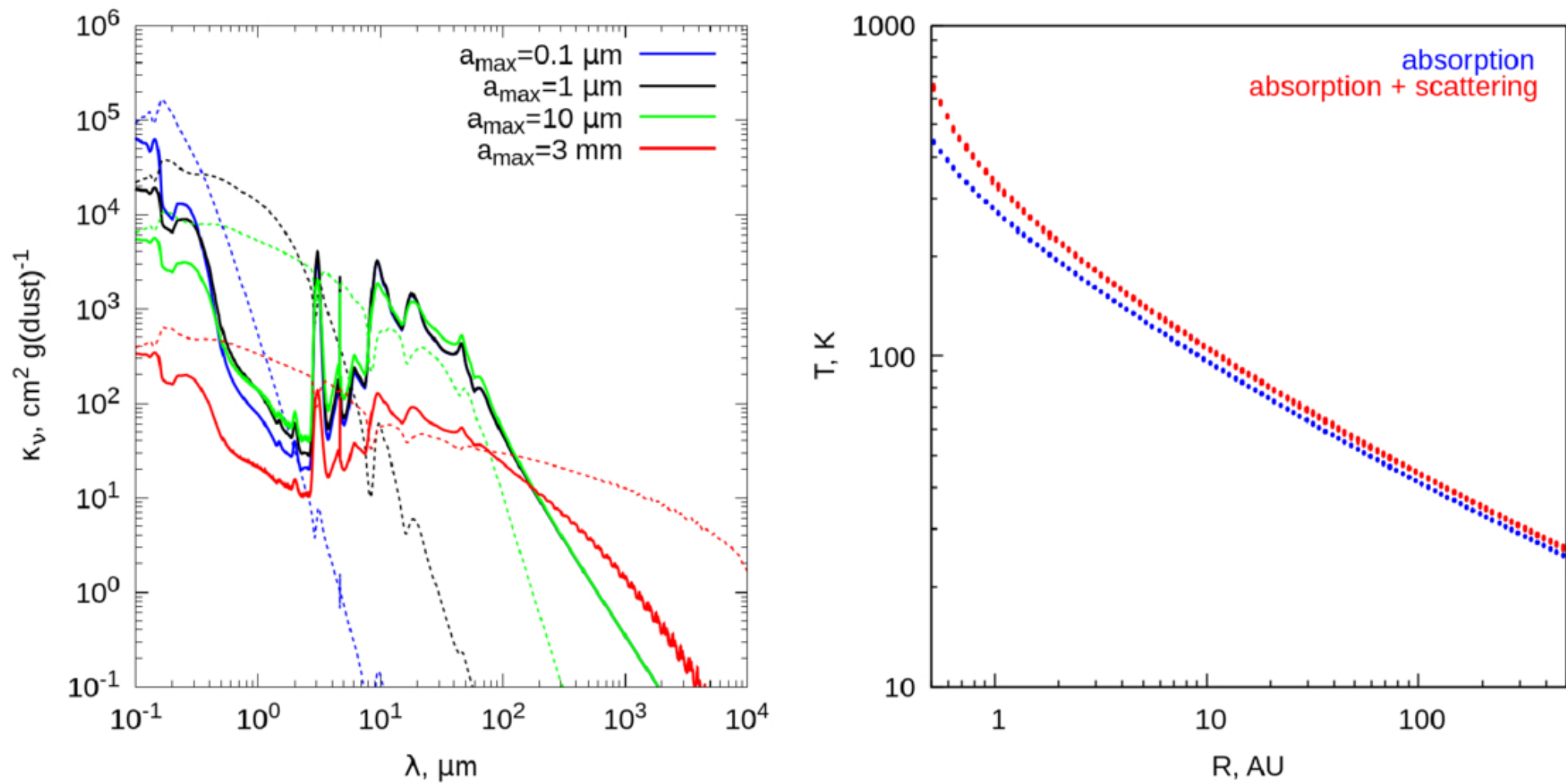
Figure 12. from Igor Petrashkevich et al 2026 Astrophys. J. 1006 doi:10.3847/1538-4357/ae7b20 https://dx.doi.org/10.3847/1538-4357/ae7b20 © 2026. The Author(s). Published by the American Astronomical Society.
