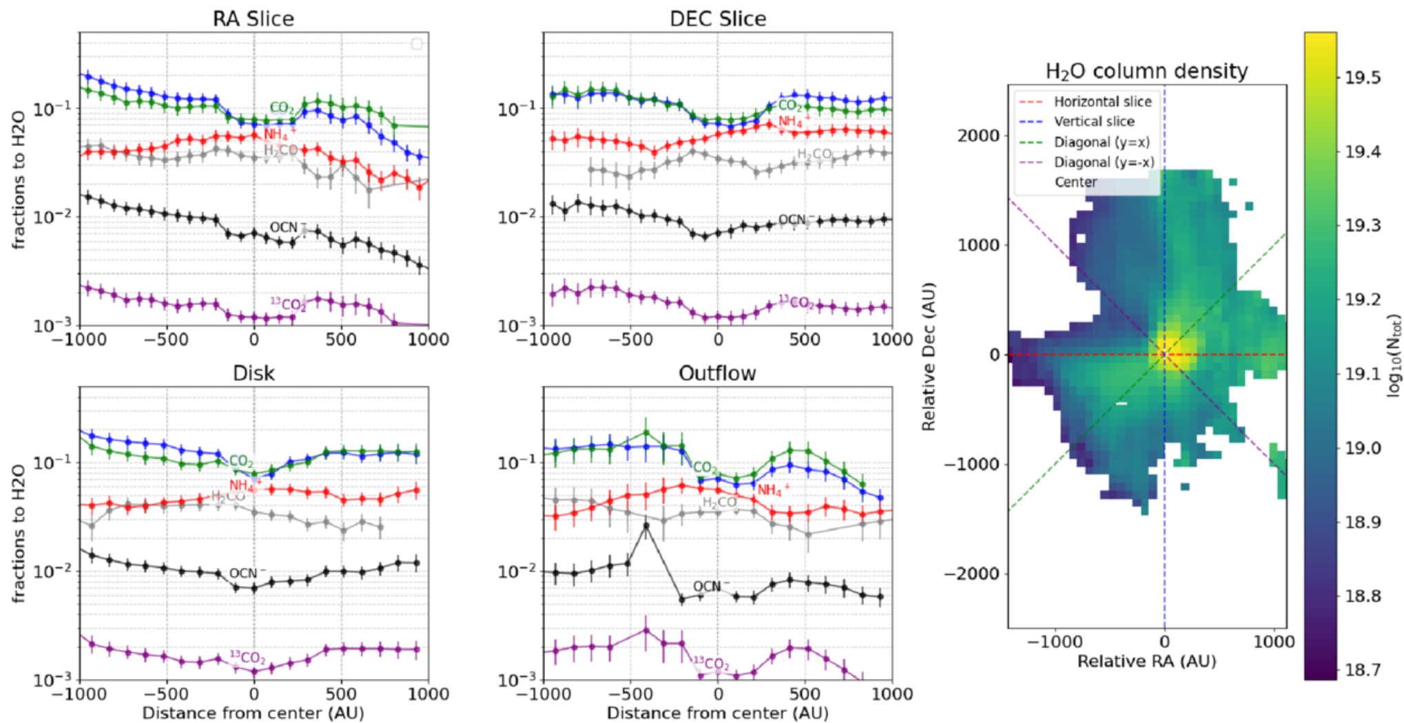
Figure 11. from Igor Petrashkevich et al 2026 Astrophys. J. 1006 doi:10.3847/1538-4357/ae7b20 https://dx.doi.org/10.3847/1538-4357/ae7b20 © 2026. The Author(s). Published by the American Astronomical Society.
