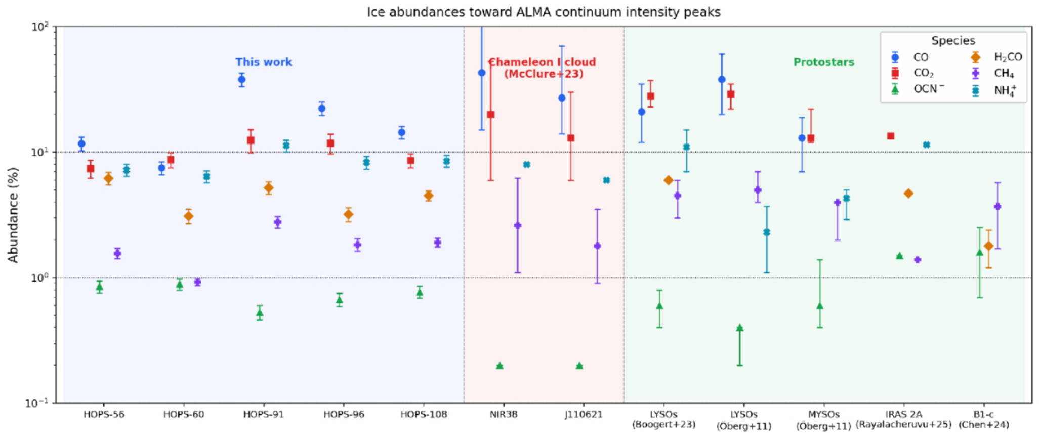
Figure 10. from Igor Petrashkevich et al 2026 Astrophys. J. 1006 doi:10.3847/1538-4357/ae7b20 https://dx.doi.org/10.3847/1538-4357/ae7b20 © 2026. The Author(s). Published by the American Astronomical Society.
