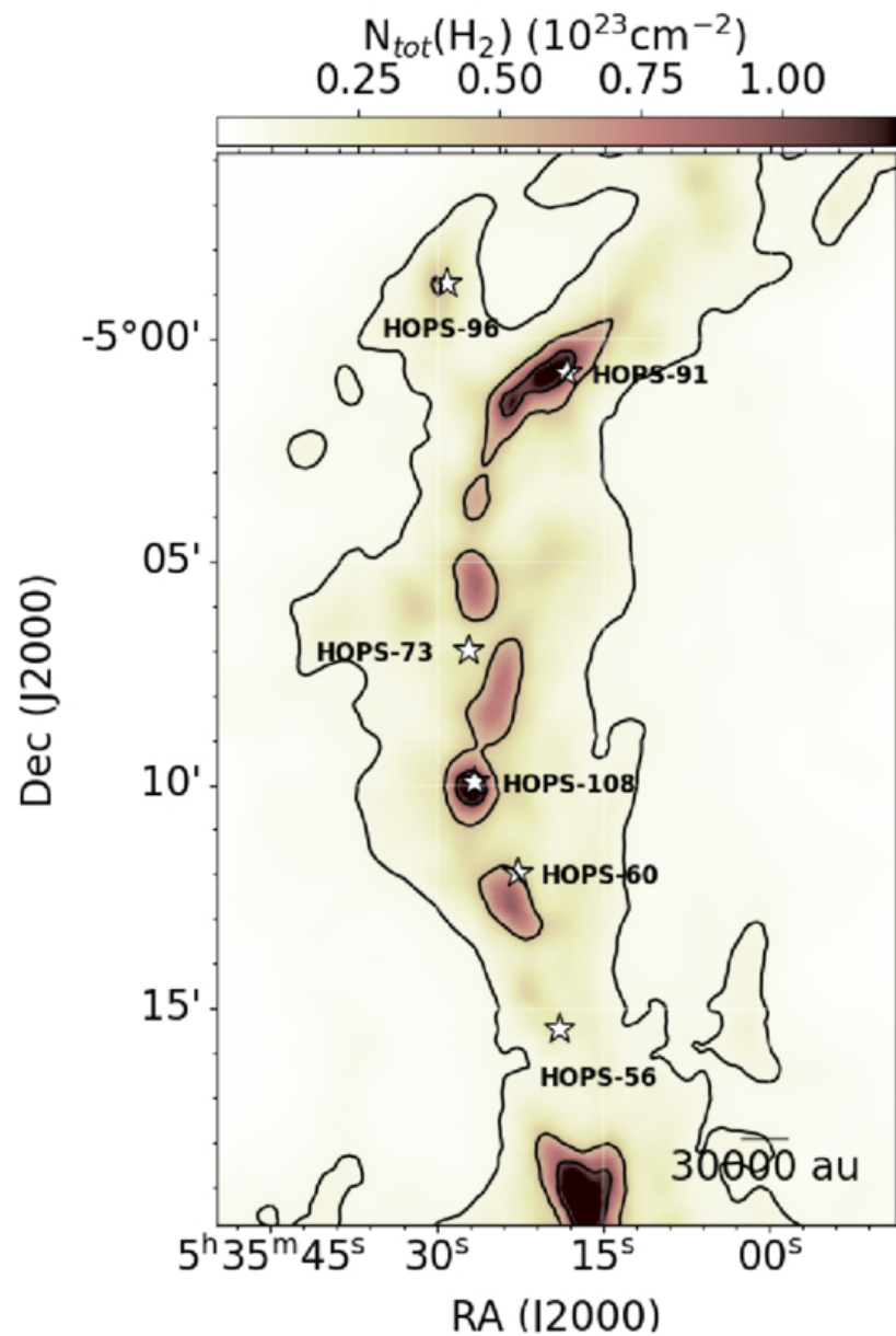
Figure 1. from Igor Petrashkevich et al 2026 Astrophys. J. 1006 doi:10.3847/1538-4357/ae7b20 https://dx.doi.org/10.3847/1538-4357/ae7b20 © 2026. The Author(s). Published by the American Astronomical Society.
