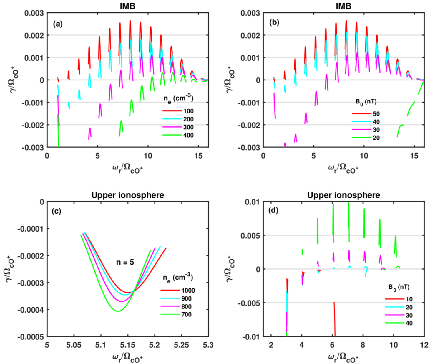
Figure 5. from Amrutha et al 2026 Astrophys. J. 1005 doi:10.3847/1538-4357/ae7a5d https://dx.doi.org/10.3847/1538-4357/ae7a5d © 2026. The Author(s). Published by the American Astronomical Society.
