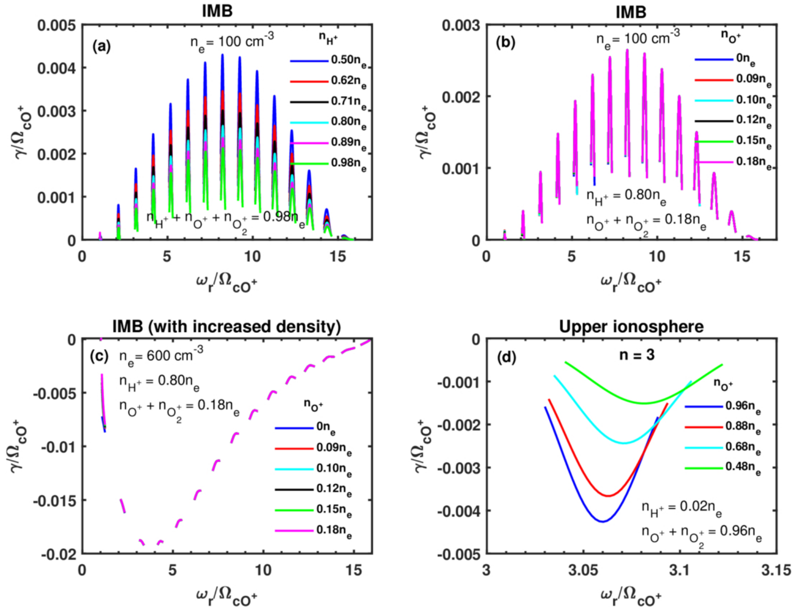
Figure 4. from Amrutha et al 2026 Astrophys. J. 1005 doi:10.3847/1538-4357/ae7a5d https://dx.doi.org/10.3847/1538-4357/ae7a5d © 2026. The Author(s). Published by the American Astronomical Society.
