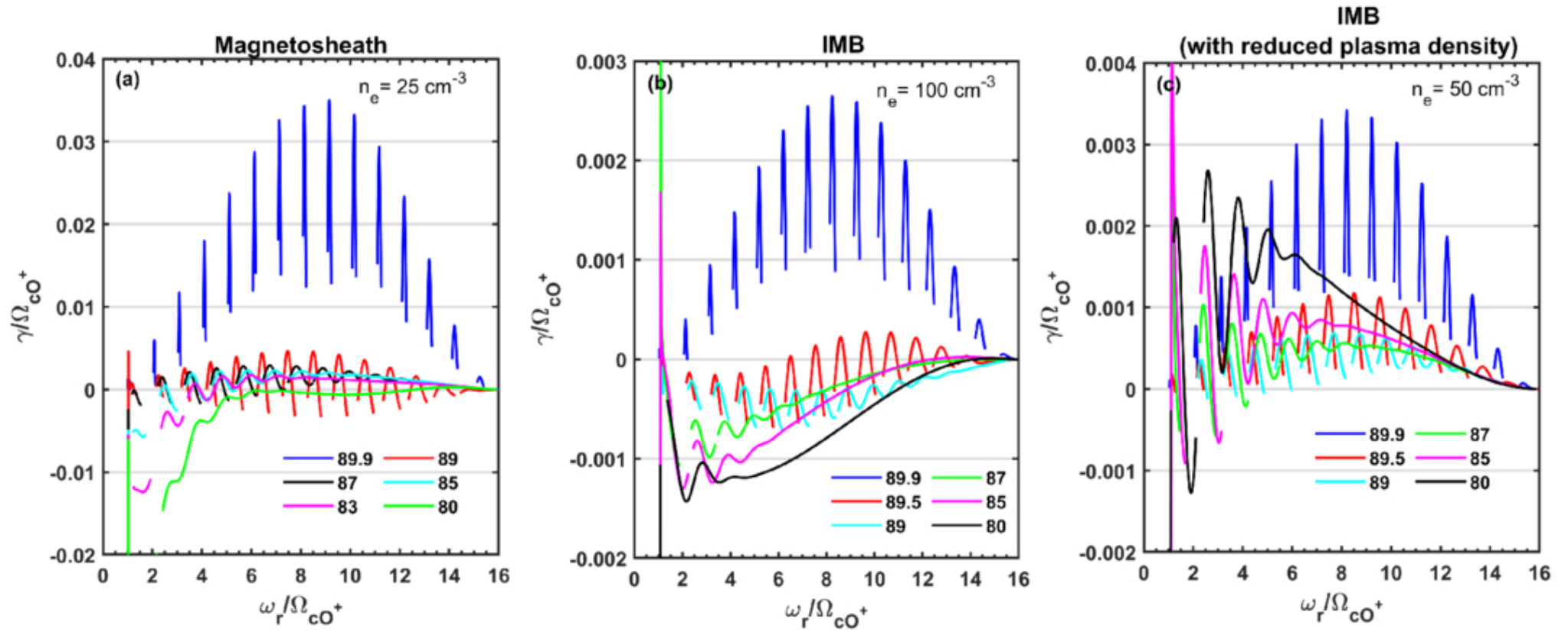
Figure 3. from Amrutha et al 2026 Astrophys. J. 1005 doi:10.3847/1538-4357/ae7a5d https://dx.doi.org/10.3847/1538-4357/ae7a5d © 2026. The Author(s). Published by the American Astronomical Society.
