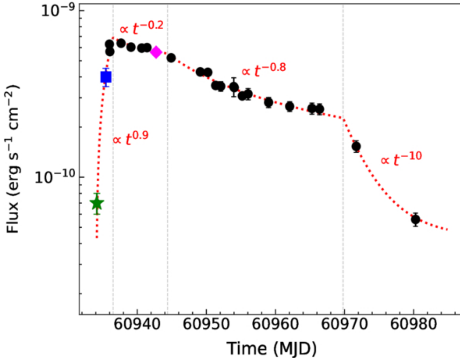
Figure 5. from Gaurava K. Jaisawal et al 2026 Astrophys. J. 1005 doi:10.3847/1538-4357/ae7a58 https://dx.doi.org/10.3847/1538-4357/ae7a58 © 2026. The Author(s). Published by the American Astronomical Society.
