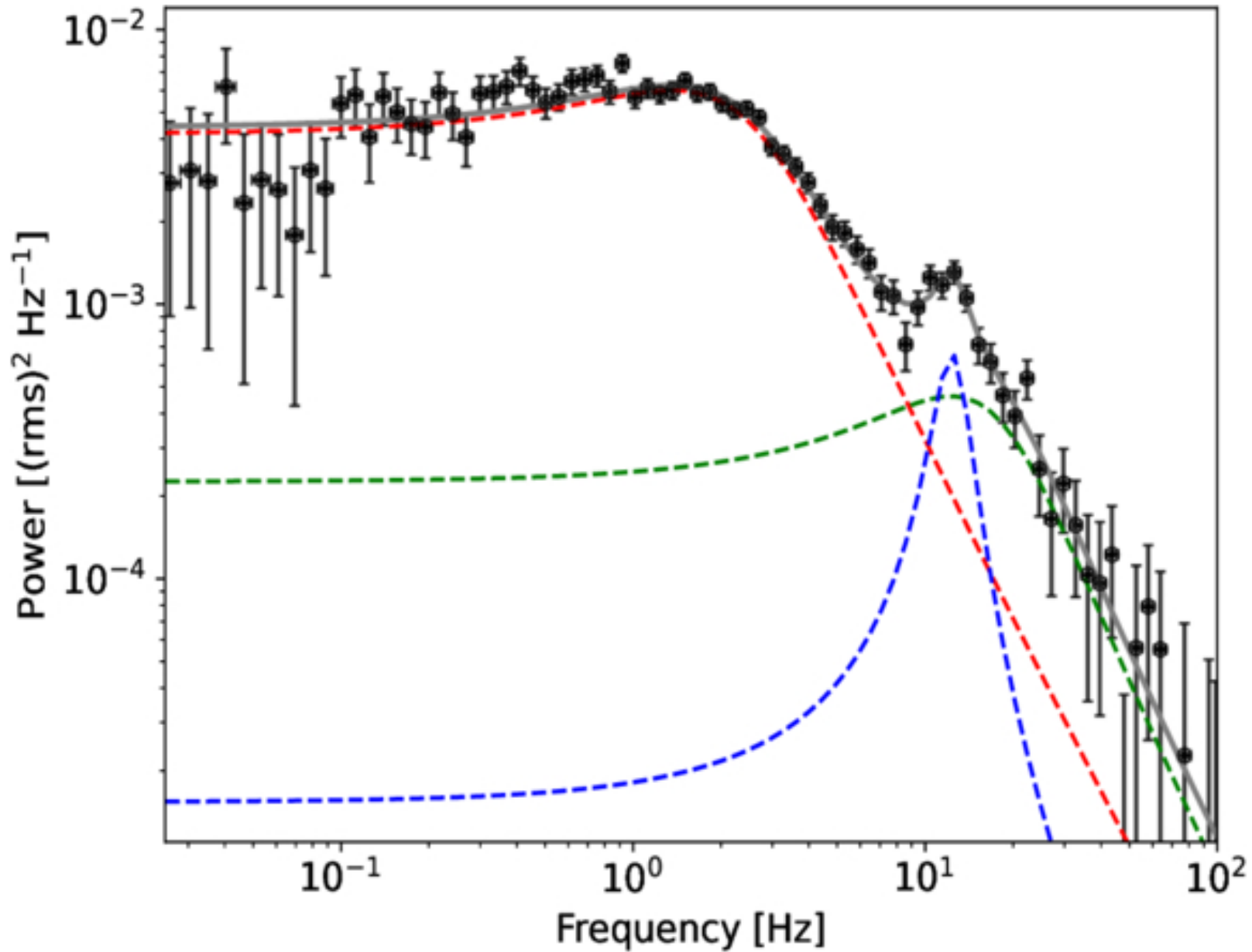
Figure 3. from Gaurava K. Jaisawal et al 2026 Astrophys. J. 1005 doi:10.3847/1538-4357/ae7a58 https://dx.doi.org/10.3847/1538-4357/ae7a58 © 2026. The Author(s). Published by the American Astronomical Society.
