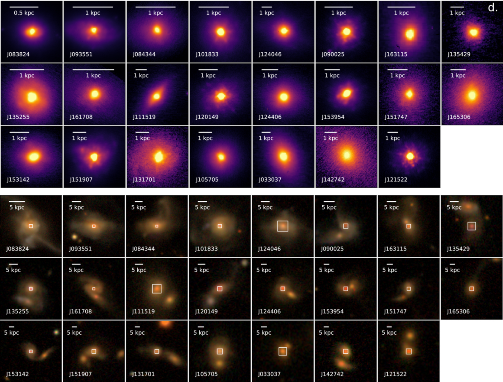
Figure 9. from Camilo Vazquez et al 2026 Astrophys. J. 1006 doi:10.3847/1538-4357/ae7a4b https://dx.doi.org/10.3847/1538-4357/ae7a4b © 2026. The Author(s). Published by the American Astronomical Society.
