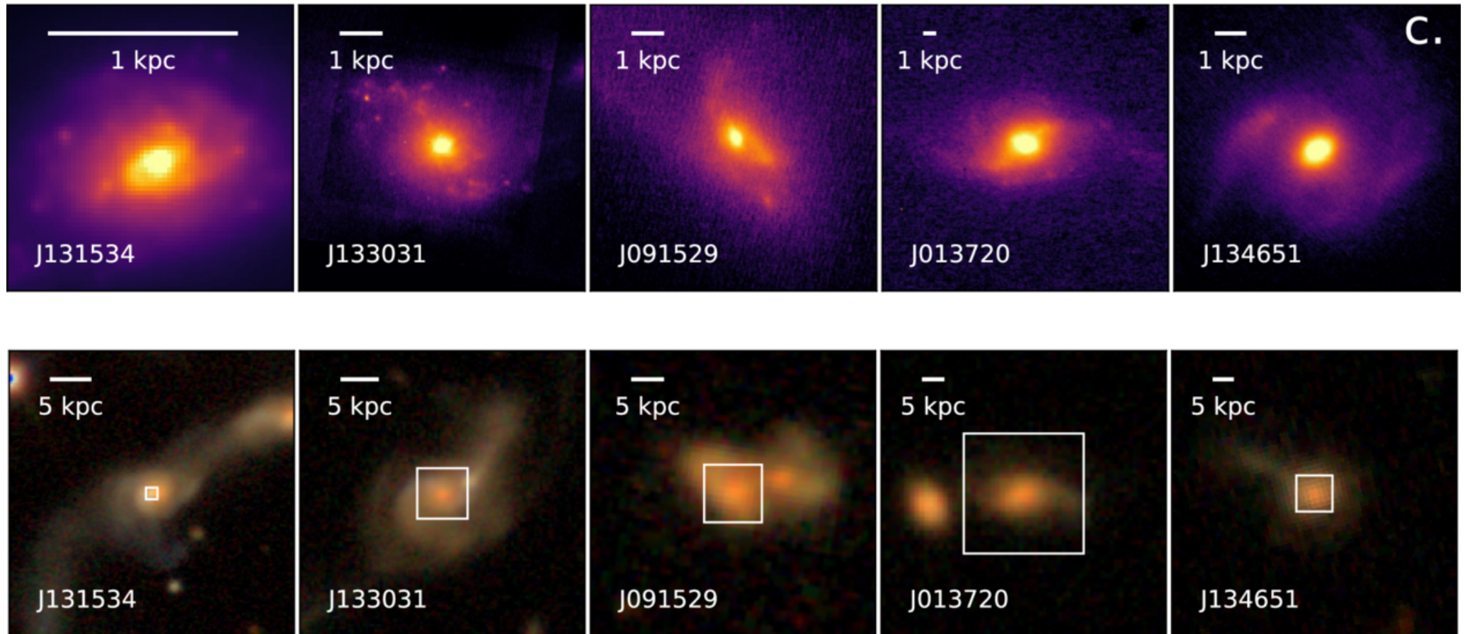
Figure 9. from Camilo Vazquez et al 2026 Astrophys. J. 1006 doi:10.3847/1538-4357/ae7a4b https://dx.doi.org/10.3847/1538-4357/ae7a4b © 2026. The Author(s). Published by the American Astronomical Society.
