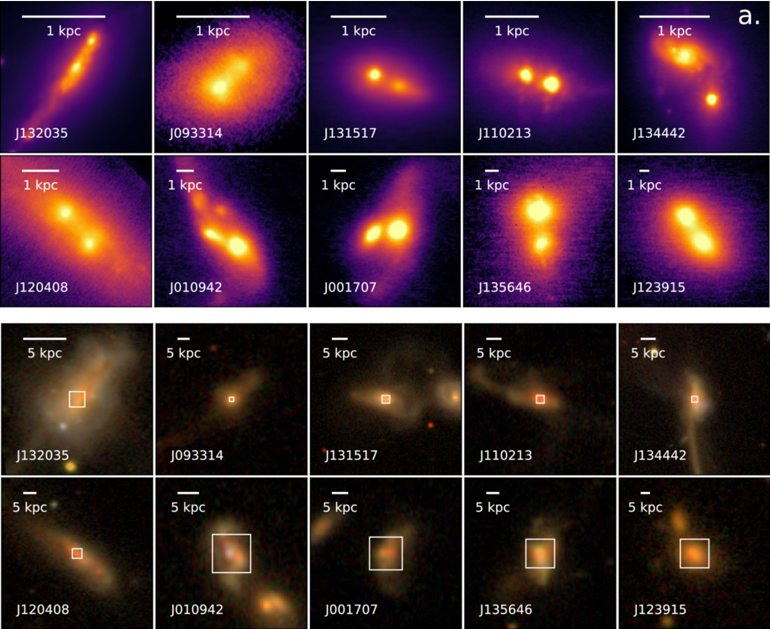
Figure 9. from Camilo Vazquez et al 2026 Astrophys. J. 1006 doi:10.3847/1538-4357/ae7a4b https://dx.doi.org/10.3847/1538-4357/ae7a4b © 2026. The Author(s). Published by the American Astronomical Society.
