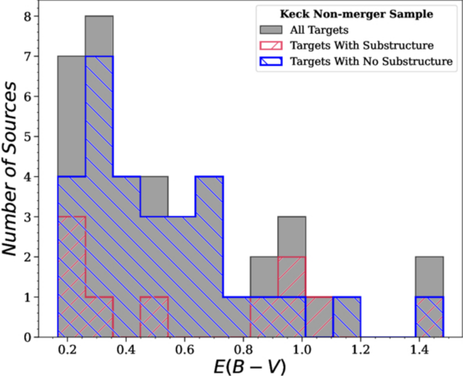
Figure 8. from Camilo Vazquez et al 2026 Astrophys. J. 1006 doi:10.3847/1538-4357/ae7a4b https://dx.doi.org/10.3847/1538-4357/ae7a4b © 2026. The Author(s). Published by the American Astronomical Society.
