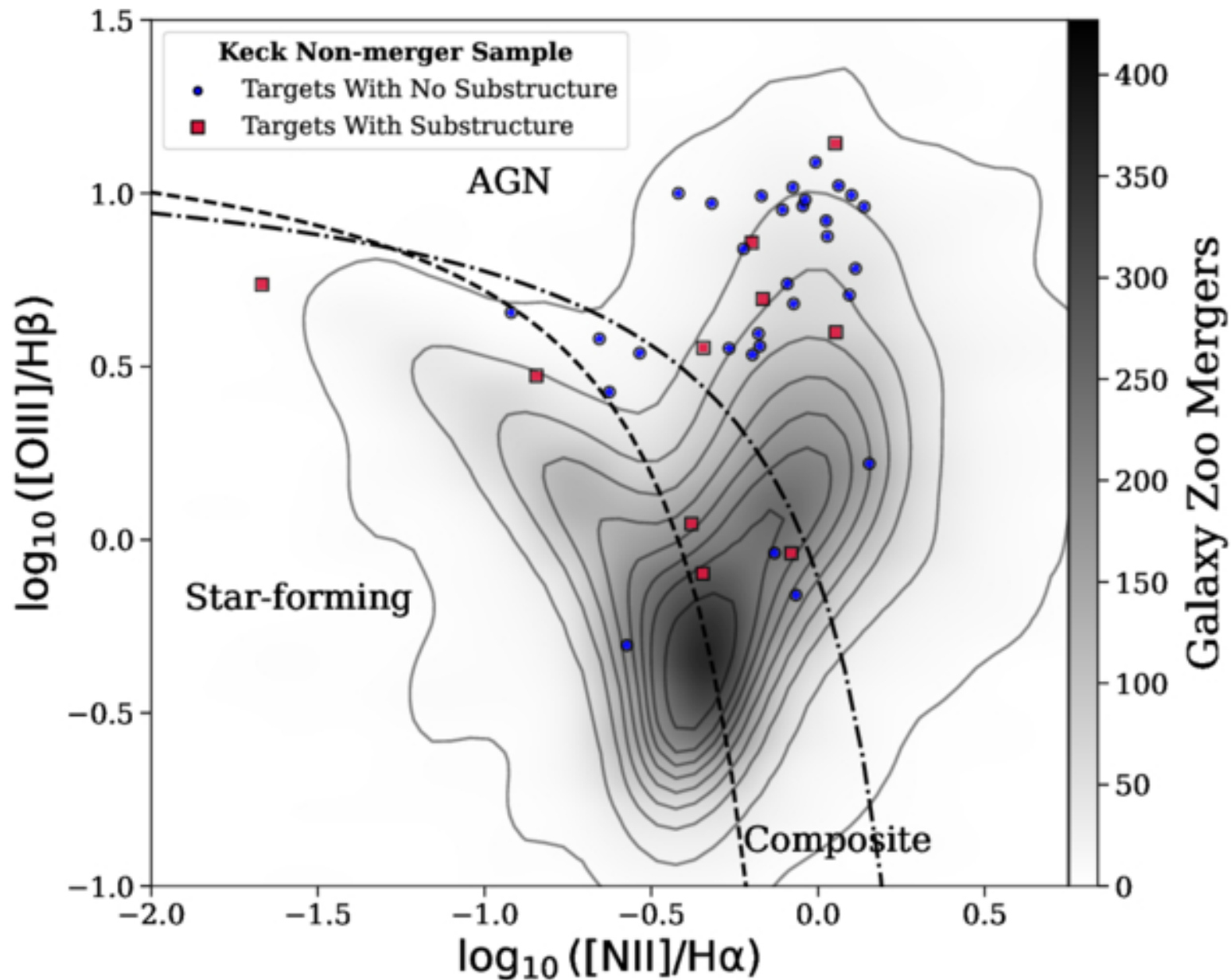
Figure 6. from Camilo Vazquez et al 2026 Astrophys. J. 1006 doi:10.3847/1538-4357/ae7a4b https://dx.doi.org/10.3847/1538-4357/ae7a4b © 2026. The Author(s). Published by the American Astronomical Society.
