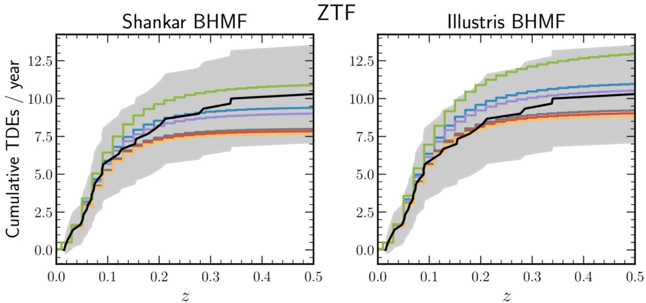
Figure 9. from Mitchell Karmen et al 2026 Astrophys. J. 1006 doi:10.3847/1538-4357/ae7a49 https://dx.doi.org/10.3847/1538-4357/ae7a49 © 2026. The Author(s). Published by the American Astronomical Society.
