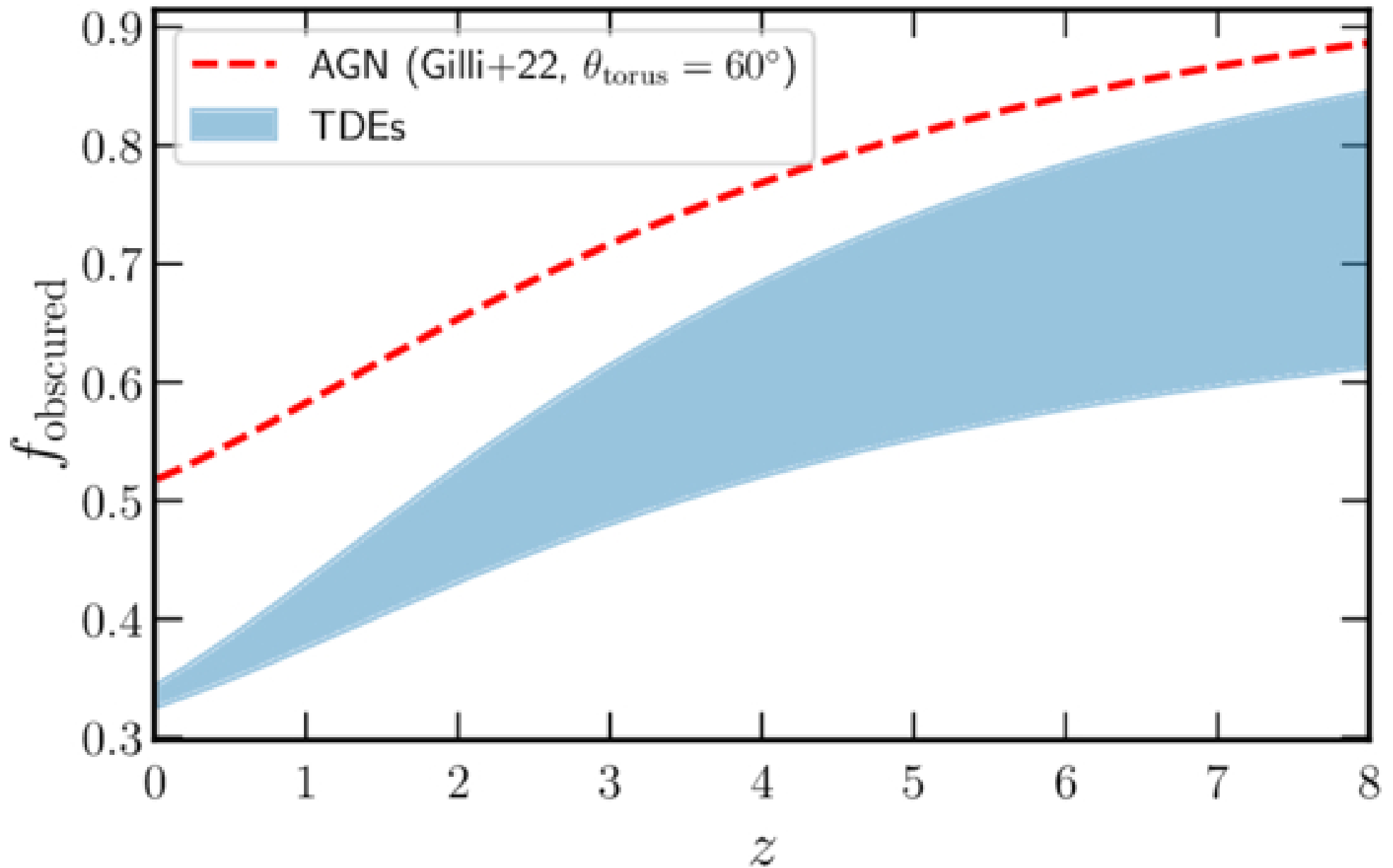
Figure 2. from Mitchell Karmen et al 2026 Astrophys. J. 1006 doi:10.3847/1538-4357/ae7a49 https://dx.doi.org/10.3847/1538-4357/ae7a49 © 2026. The Author(s). Published by the American Astronomical Society.
