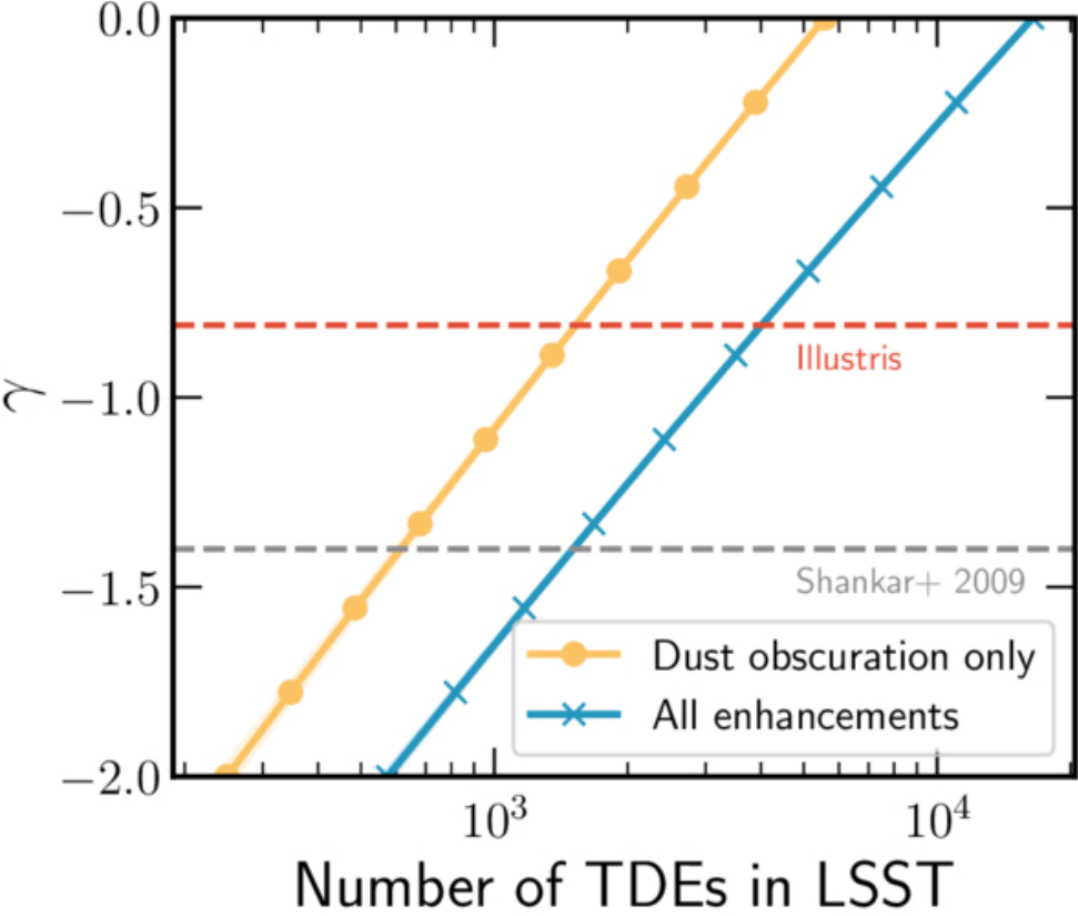
Figure 11. from Mitchell Karmen et al 2026 Astrophys. J. 1006 doi:10.3847/1538-4357/ae7a49 https://dx.doi.org/10.3847/1538-4357/ae7a49 © 2026. The Author(s). Published by the American Astronomical Society.
