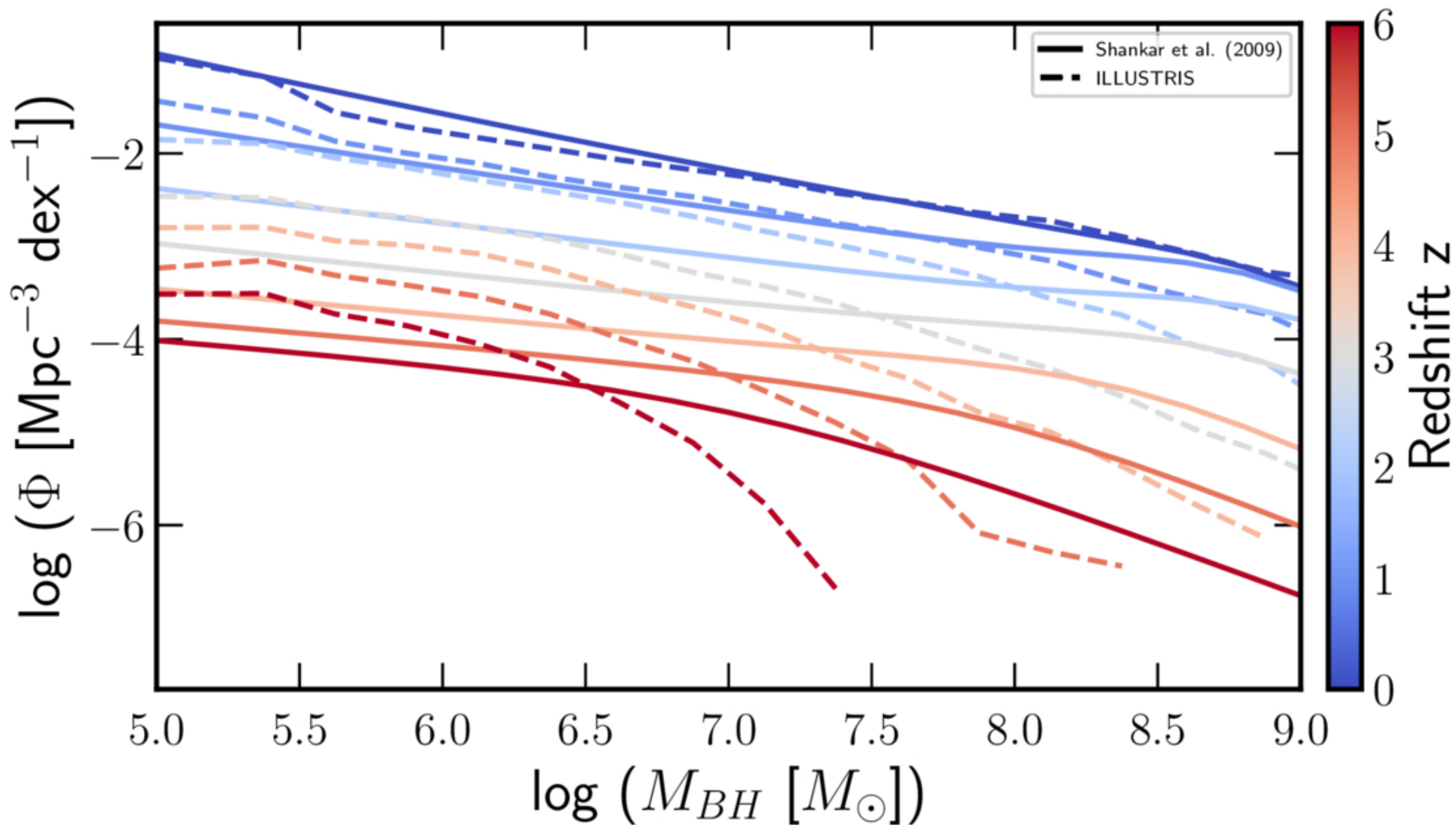
Figure 1. from Mitchell Karmen et al 2026 Astrophys. J. 1006 doi:10.3847/1538-4357/ae7a49 https://dx.doi.org/10.3847/1538-4357/ae7a49 © 2026. The Author(s). Published by the American Astronomical Society.
