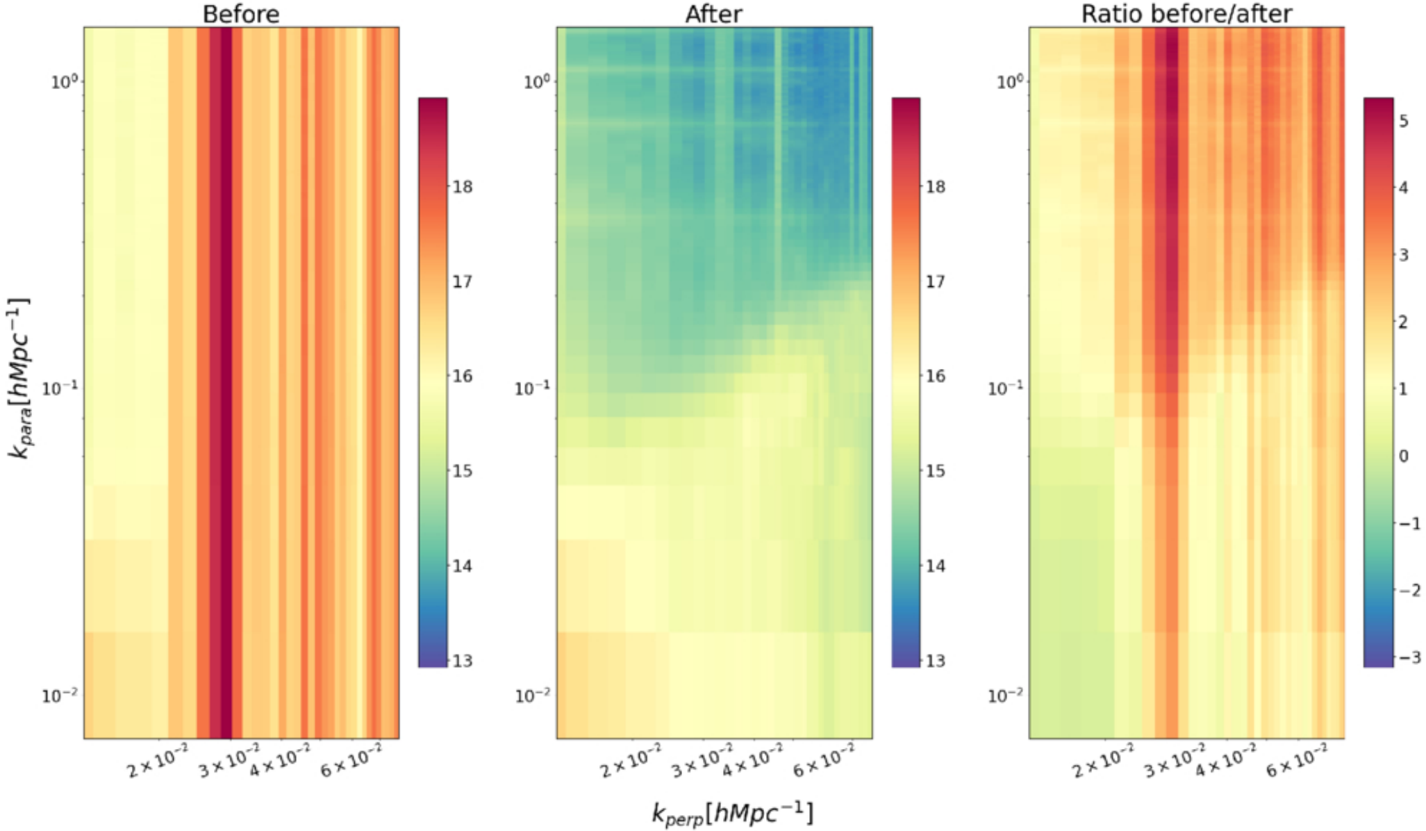
Figure 9. from Wildan Hidayat et al 2026 Astrophys. J. 1006 doi:10.3847/1538-4357/ae7a3b https://dx.doi.org/10.3847/1538-4357/ae7a3b © 2026. The Author(s). Published by the American Astronomical Society.
