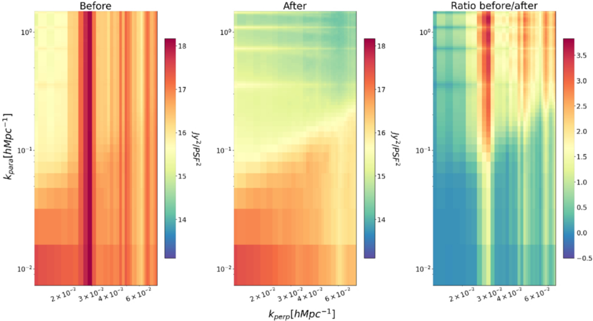
Figure 8. from Wildan Hidayat et al 2026 Astrophys. J. 1006 doi:10.3847/1538-4357/ae7a3b https://dx.doi.org/10.3847/1538-4357/ae7a3b © 2026. The Author(s). Published by the American Astronomical Society.
