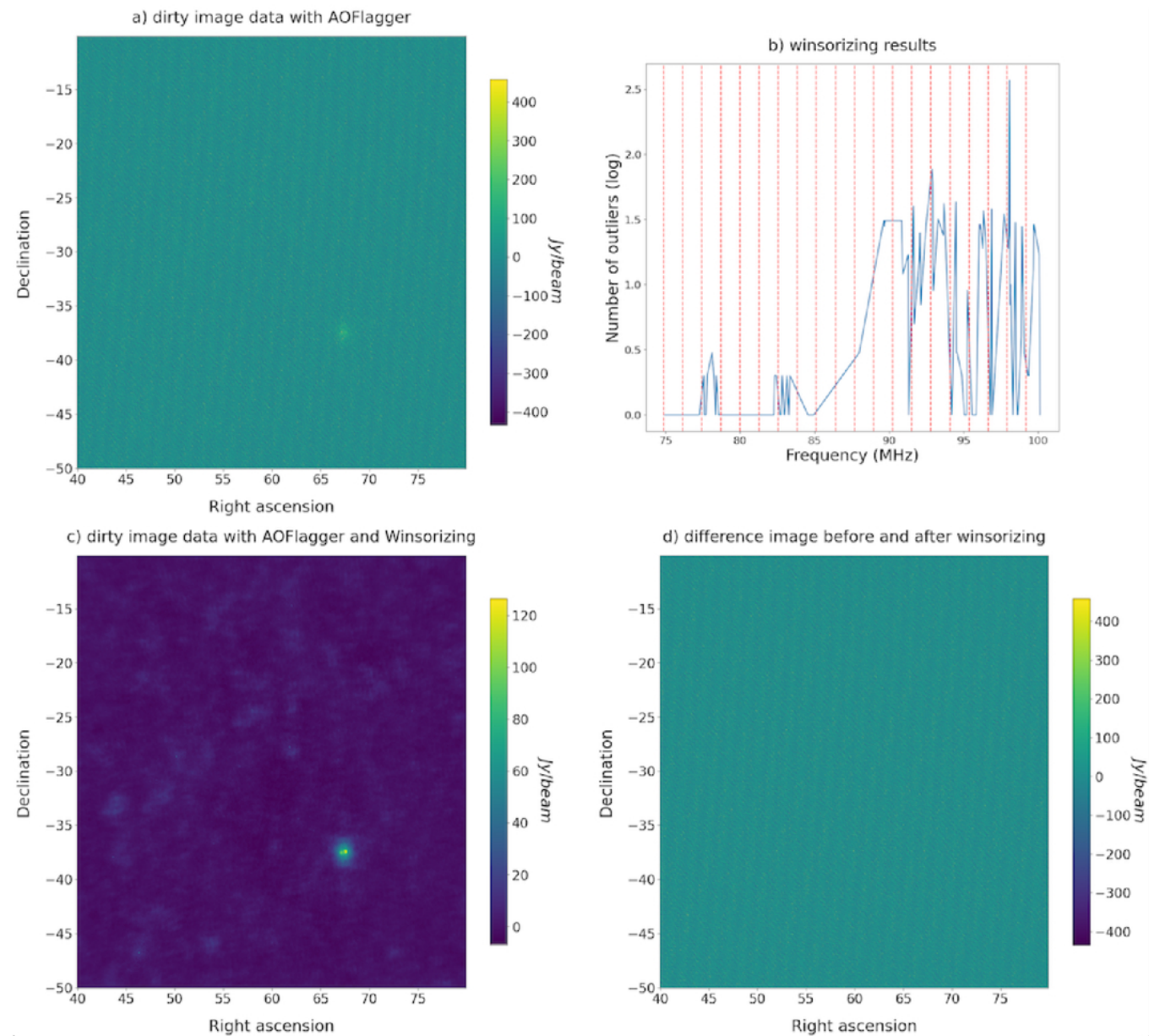
Figure 7. from Wildan Hidayat et al 2026 Astrophys. J. 1006 doi:10.3847/1538-4357/ae7a3b https://dx.doi.org/10.3847/1538-4357/ae7a3b © 2026. The Author(s). Published by the American Astronomical Society.
