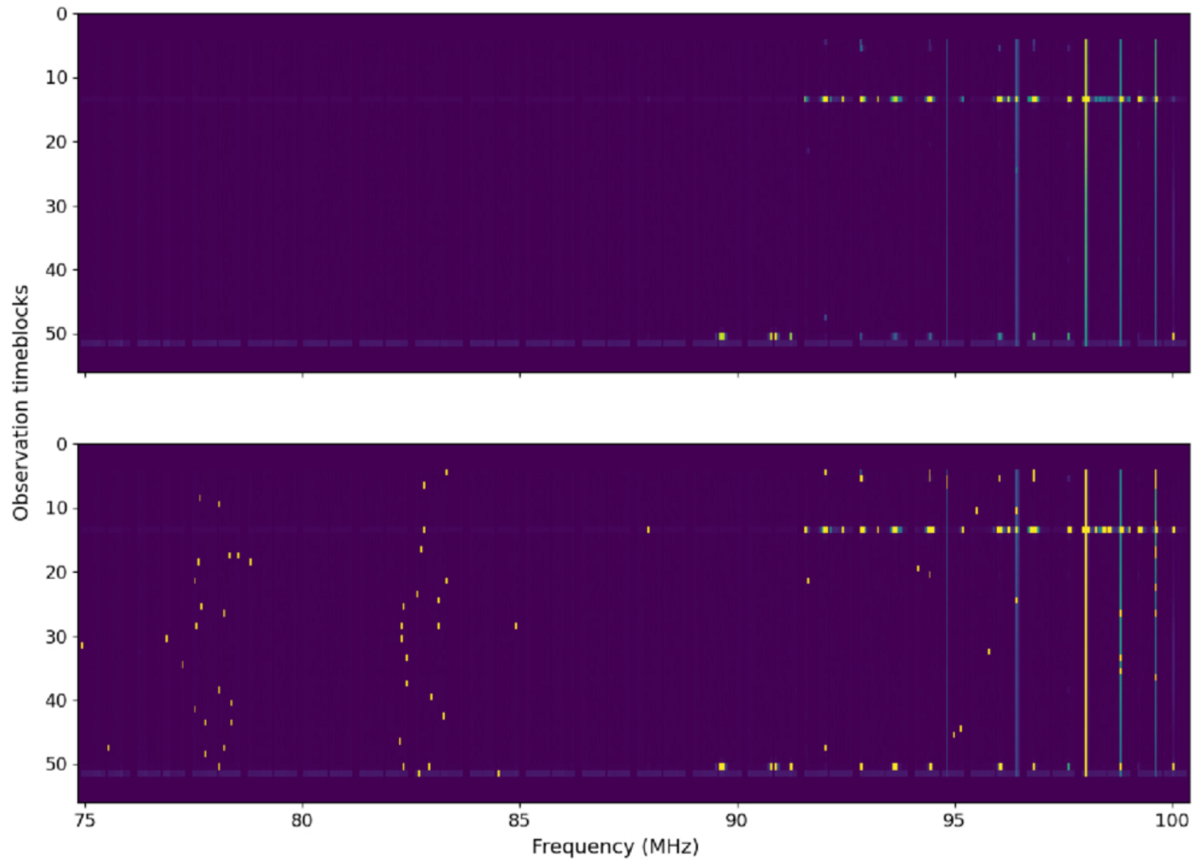
Figure 6. from Wildan Hidayat et al 2026 Astrophys. J. 1006 doi:10.3847/1538-4357/ae7a3b https://dx.doi.org/10.3847/1538-4357/ae7a3b © 2026. The Author(s). Published by the American Astronomical Society.
