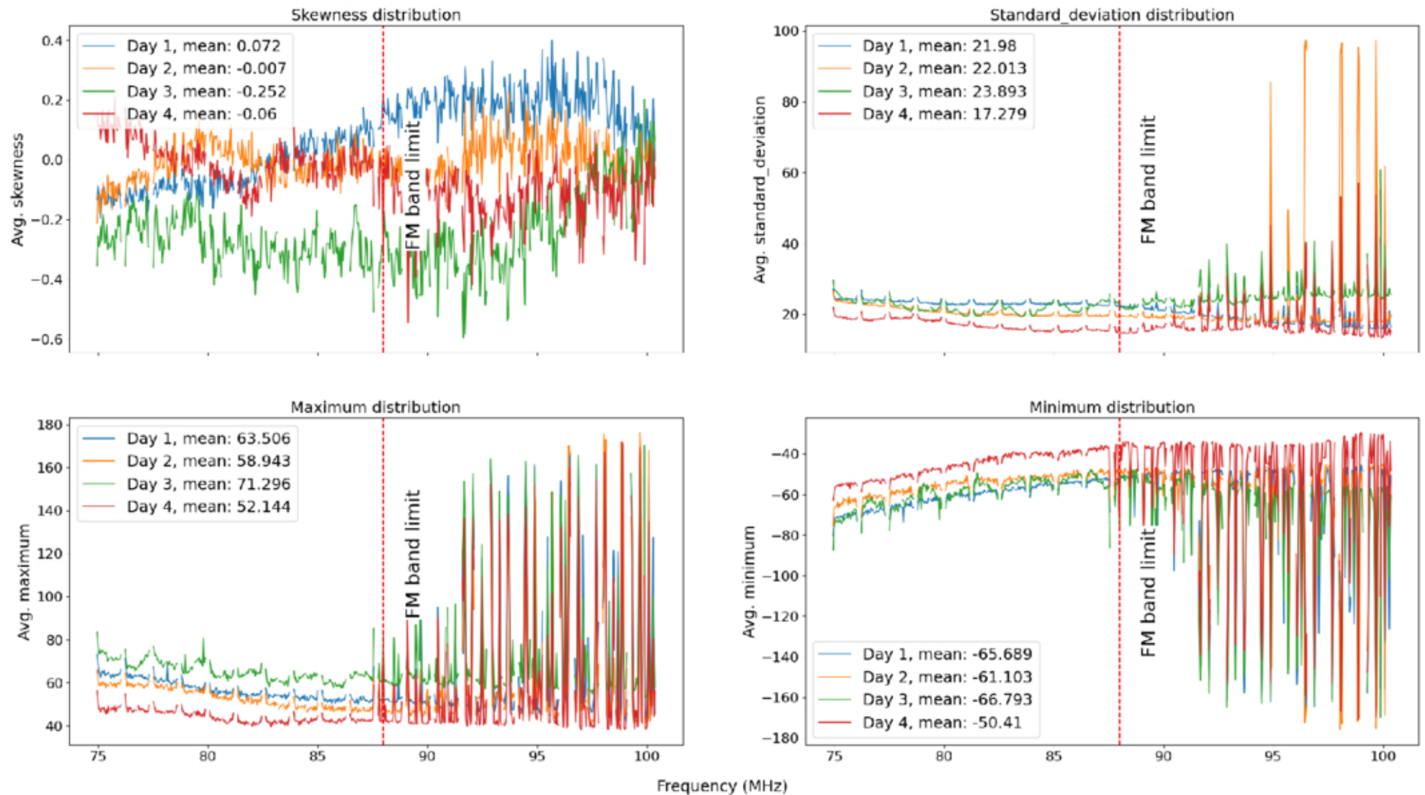
Figure 4. from Wildan Hidayat et al 2026 Astrophys. J. 1006 doi:10.3847/1538-4357/ae7a3b https://dx.doi.org/10.3847/1538-4357/ae7a3b © 2026. The Author(s). Published by the American Astronomical Society.
