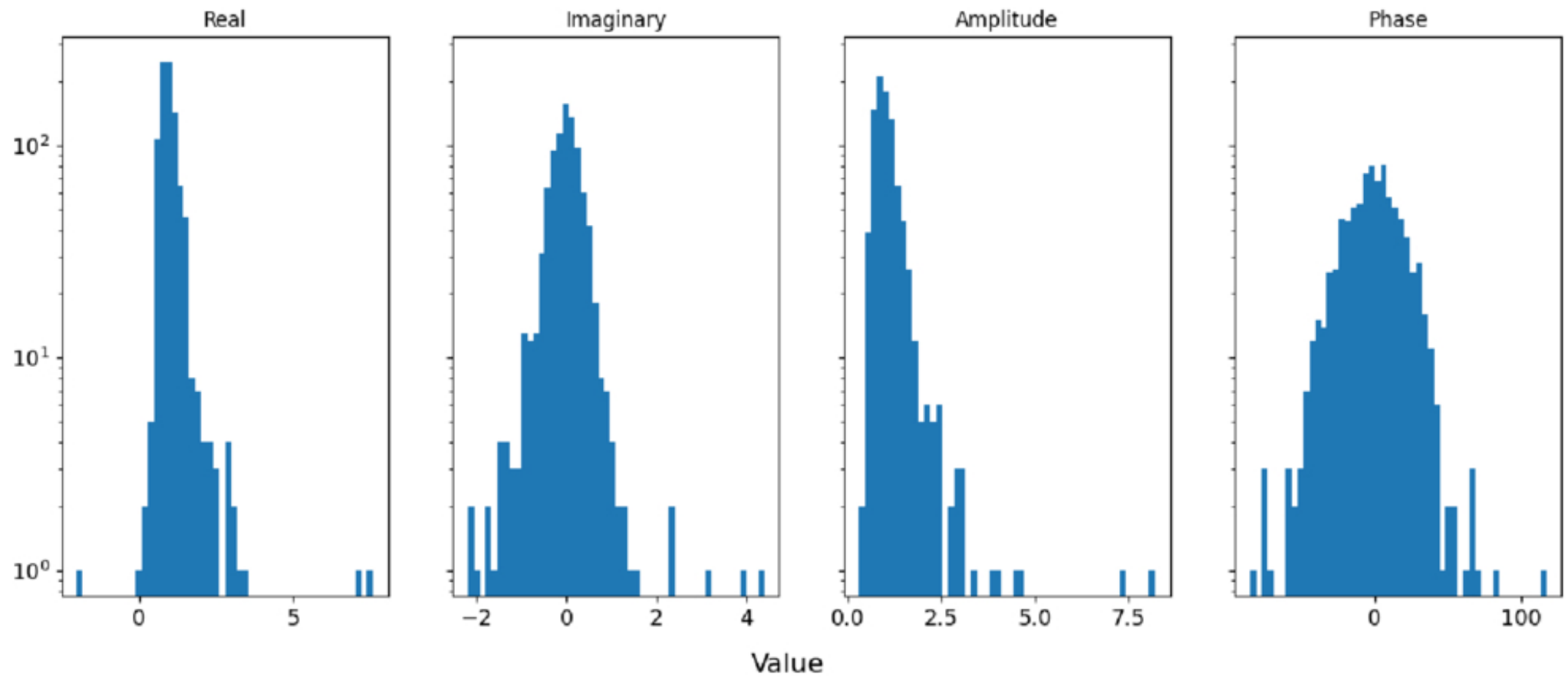
Figure 2. from Wildan Hidayat et al 2026 Astrophys. J. 1006 doi:10.3847/1538-4357/ae7a3b https://dx.doi.org/10.3847/1538-4357/ae7a3b © 2026. The Author(s). Published by the American Astronomical Society.
