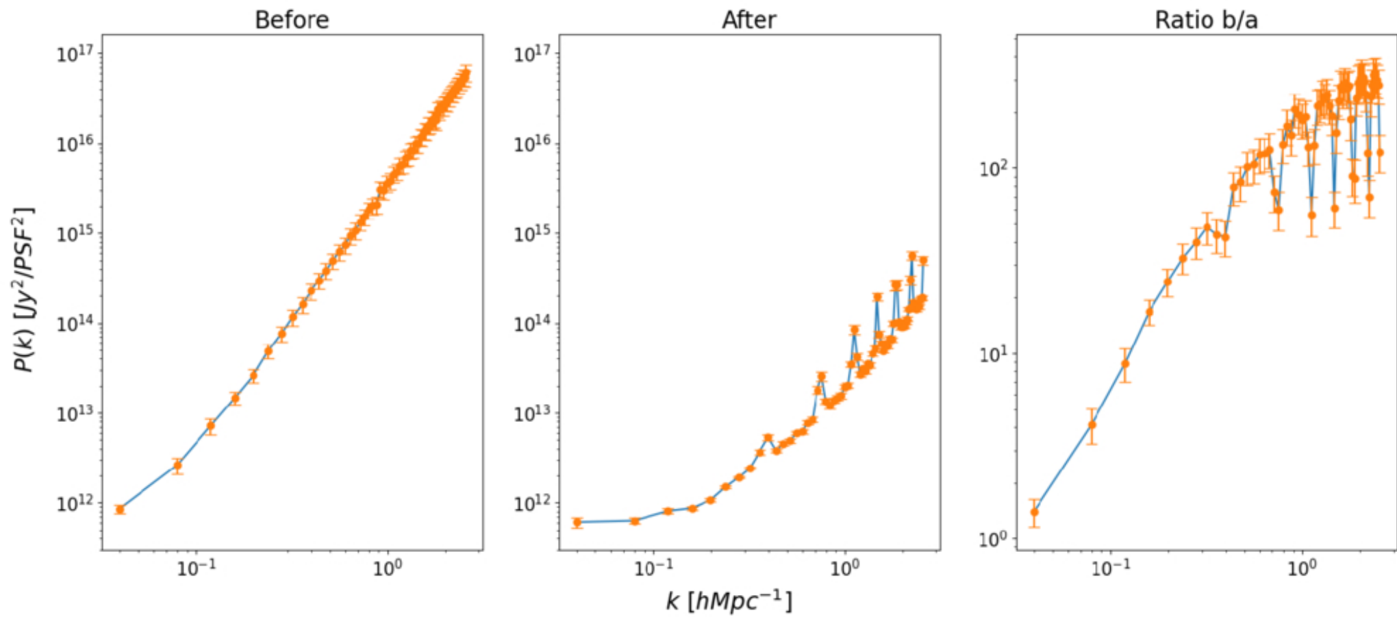
Figure 10. from Wildan Hidayat et al 2026 Astrophys. J. 1006 doi:10.3847/1538-4357/ae7a3b https://dx.doi.org/10.3847/1538-4357/ae7a3b © 2026. The Author(s). Published by the American Astronomical Society.
