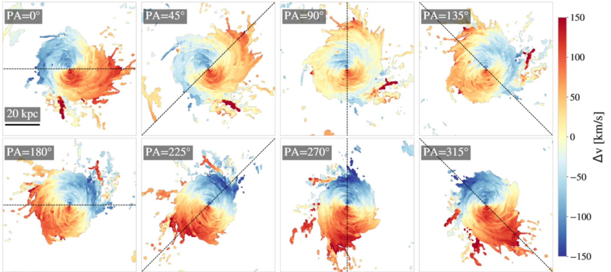
Figure 9. from Cameron W. Trapp et al 2026 Astrophys. J. 1005 doi:10.3847/1538-4357/ae7a38 https://dx.doi.org/10.3847/1538-4357/ae7a38 © 2026. The Author(s). Published by the American Astronomical Society.
