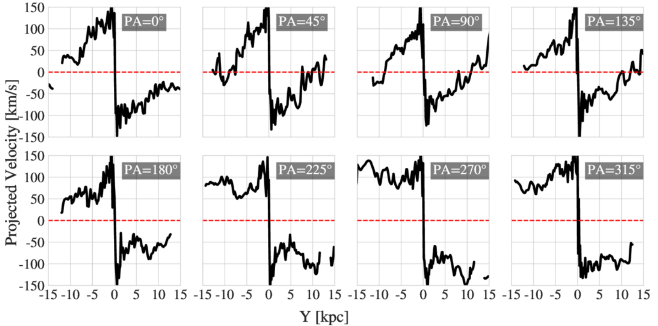
Figure 10. from Cameron W. Trapp et al 2026 Astrophys. J. 1005 doi:10.3847/1538-4357/ae7a38 https://dx.doi.org/10.3847/1538-4357/ae7a38 © 2026. The Author(s). Published by the American Astronomical Society.
