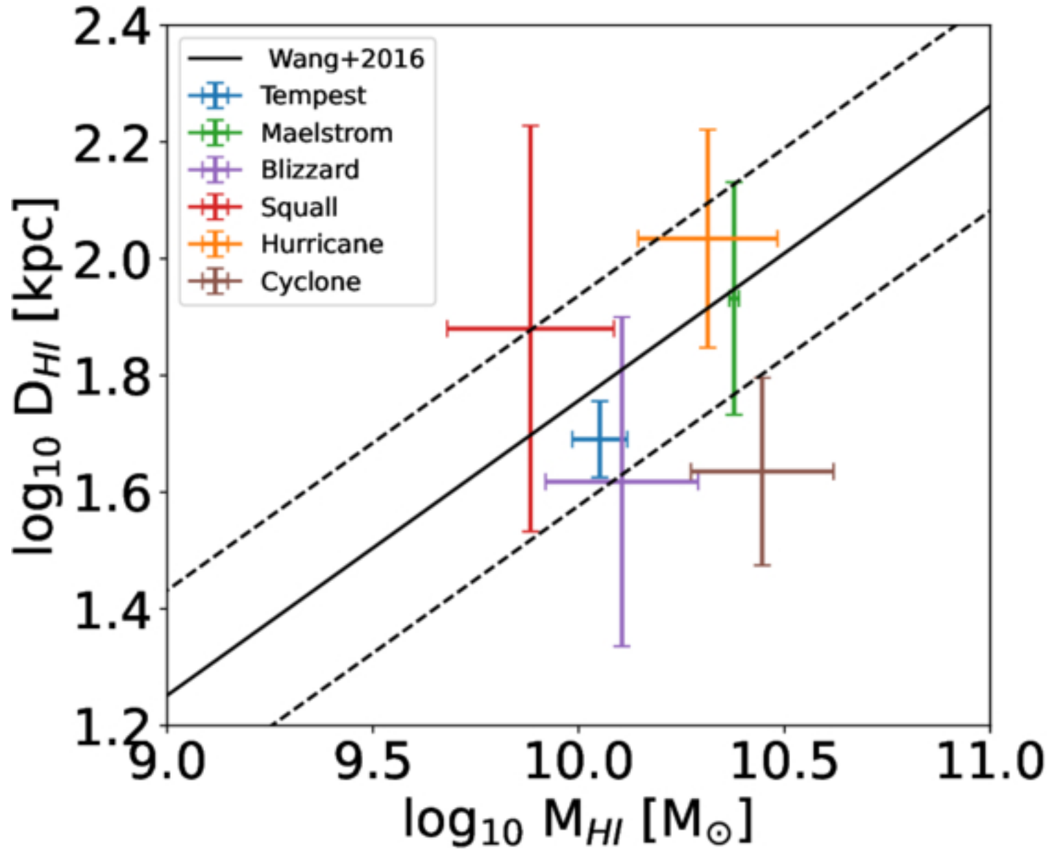
Figure 1. from Cameron W. Trapp et al 2026 Astrophys. J. 1005 doi:10.3847/1538-4357/ae7a38 https://dx.doi.org/10.3847/1538-4357/ae7a38 © 2026. The Author(s). Published by the American Astronomical Society.
