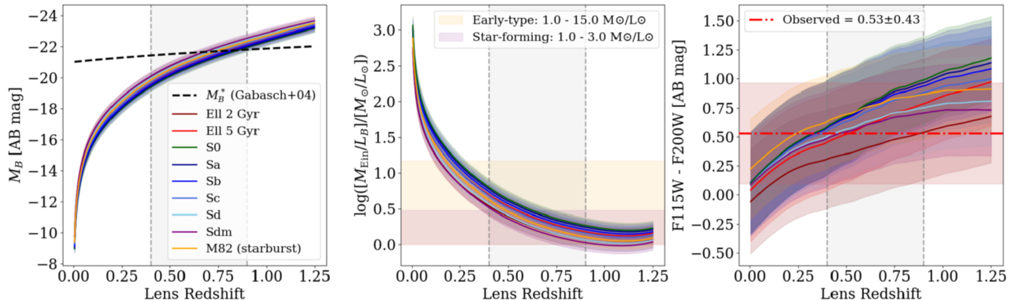
Figure 9. from Mingrui Liu et al 2026 Astrophys. J. 1006 doi:10.3847/1538-4357/ae7a37 https://dx.doi.org/10.3847/1538-4357/ae7a37 © 2026. The Author(s). Published by the American Astronomical Society.
