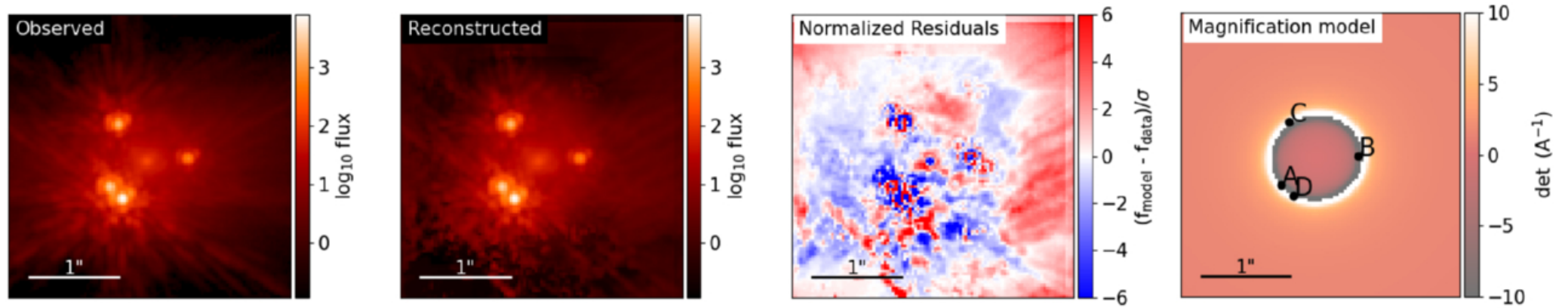
Figure 6. from Mingrui Liu et al 2026 Astrophys. J. 1006 doi:10.3847/1538-4357/ae7a37 https://dx.doi.org/10.3847/1538-4357/ae7a37 © 2026. The Author(s). Published by the American Astronomical Society.
