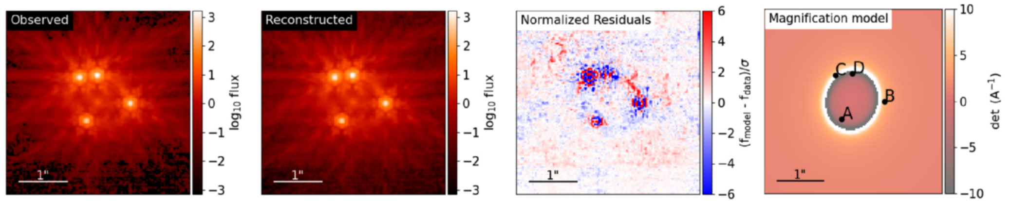
Figure 5. from Mingrui Liu et al 2026 Astrophys. J. 1006 doi:10.3847/1538-4357/ae7a37 https://dx.doi.org/10.3847/1538-4357/ae7a37 © 2026. The Author(s). Published by the American Astronomical Society.
