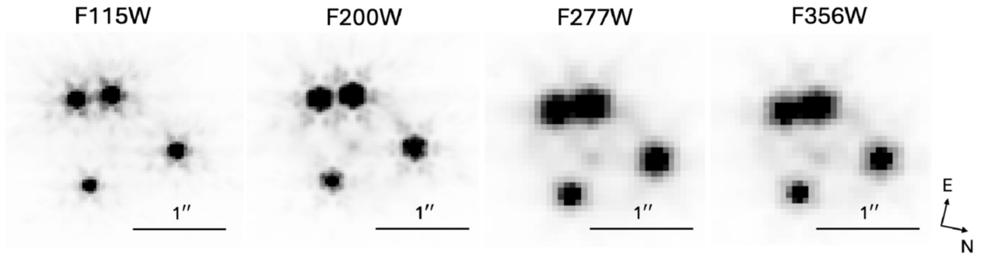
Figure 2. from Mingrui Liu et al 2026 Astrophys. J. 1006 doi:10.3847/1538-4357/ae7a37 https://dx.doi.org/10.3847/1538-4357/ae7a37 © 2026. The Author(s). Published by the American Astronomical Society.
