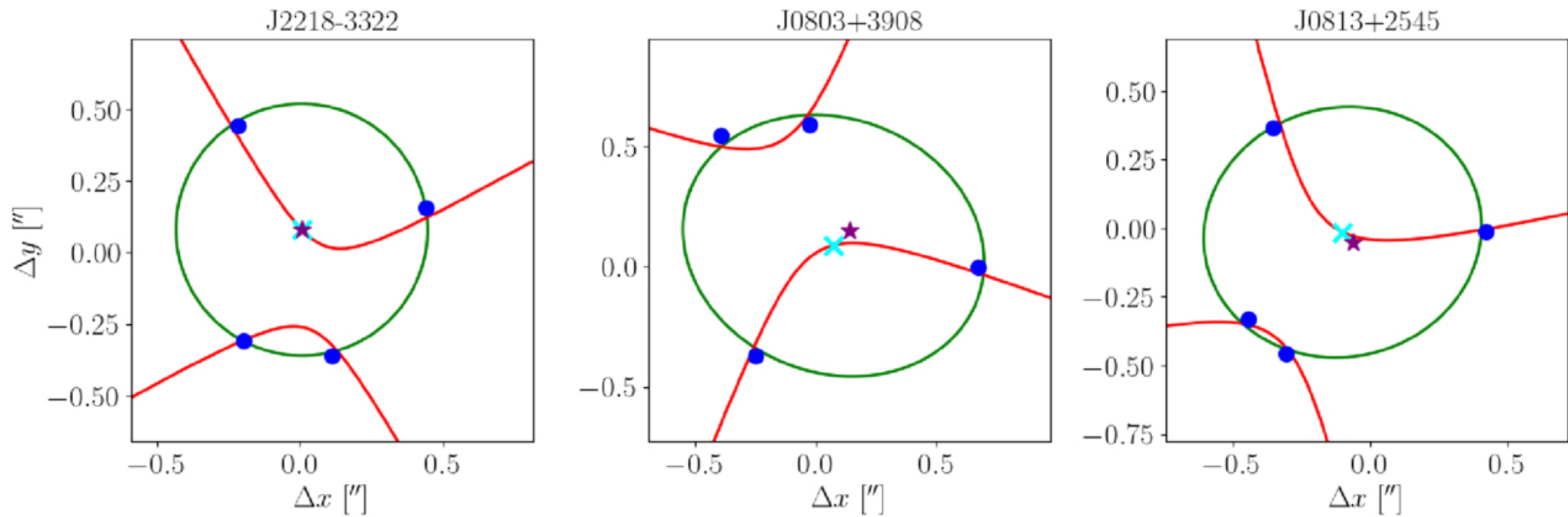
Figure 10. from Mingrui Liu et al 2026 Astrophys. J. 1006 doi:10.3847/1538-4357/ae7a37 https://dx.doi.org/10.3847/1538-4357/ae7a37 © 2026. The Author(s). Published by the American Astronomical Society.
