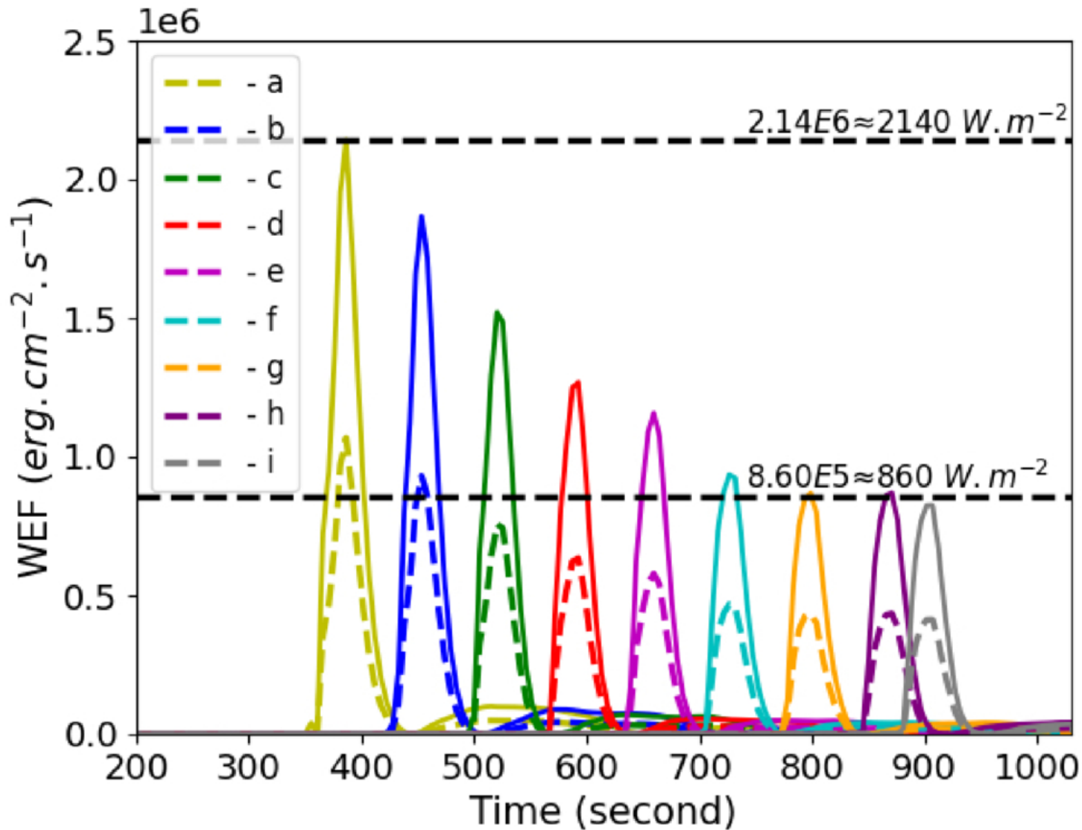
Figure 7. from Akash Bairagi et al 2026 Astrophys. J. 1005 doi:10.3847/1538-4357/ae7a36 https://dx.doi.org/10.3847/1538-4357/ae7a36 © 2026. The Author(s). Published by the American Astronomical Society.
