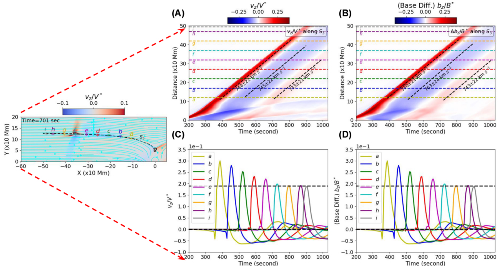
Figure 5. from Akash Bairagi et al 2026 Astrophys. J. 1005 doi:10.3847/1538-4357/ae7a36 https://dx.doi.org/10.3847/1538-4357/ae7a36 © 2026. The Author(s). Published by the American Astronomical Society.
