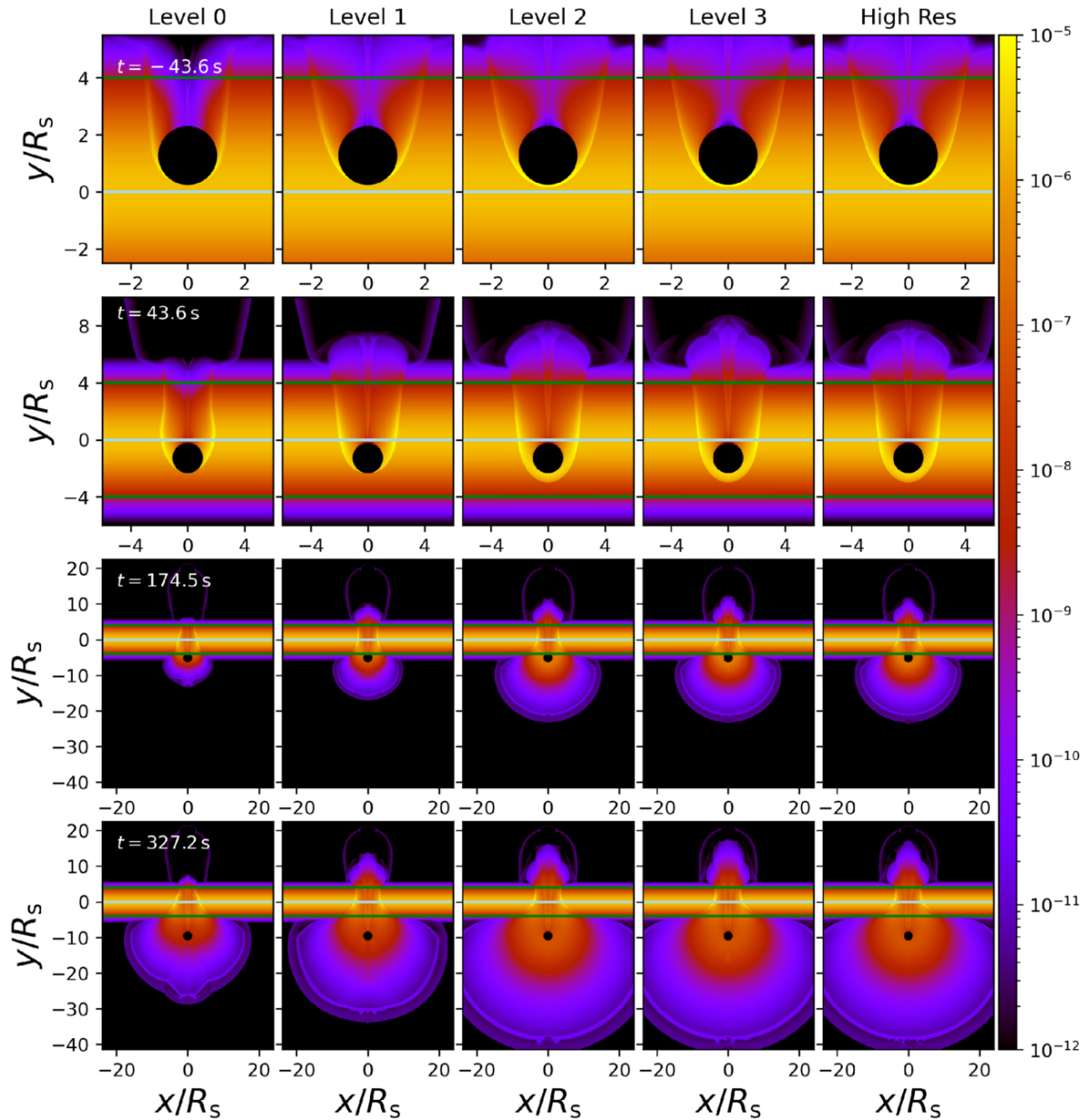
Figure 5. from Shunquan Huang et al 2026 Astrophys. J. 1005 doi:10.3847/1538-4357/ae78d4 https://dx.doi.org/10.3847/1538-4357/ae78d4 © 2026. The Author(s). Published by the American Astronomical Society.
