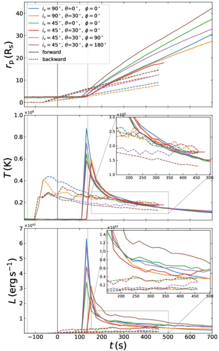
Figure 14. from Shunquan Huang et al 2026 Astrophys. J. 1005 doi:10.3847/1538-4357/ae78d4 https://dx.doi.org/10.3847/1538-4357/ae78d4 © 2026. The Author(s). Published by the American Astronomical Society.
