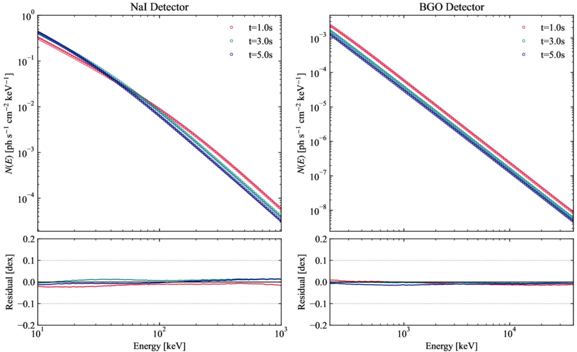
Figure 5. from Jia-Ming Chen et al 2026 Astrophys. J. 1005 doi:10.3847/1538-4357/ae78c7 https://dx.doi.org/10.3847/1538-4357/ae78c7 © 2026. The Author(s). Published by the American Astronomical Society.
