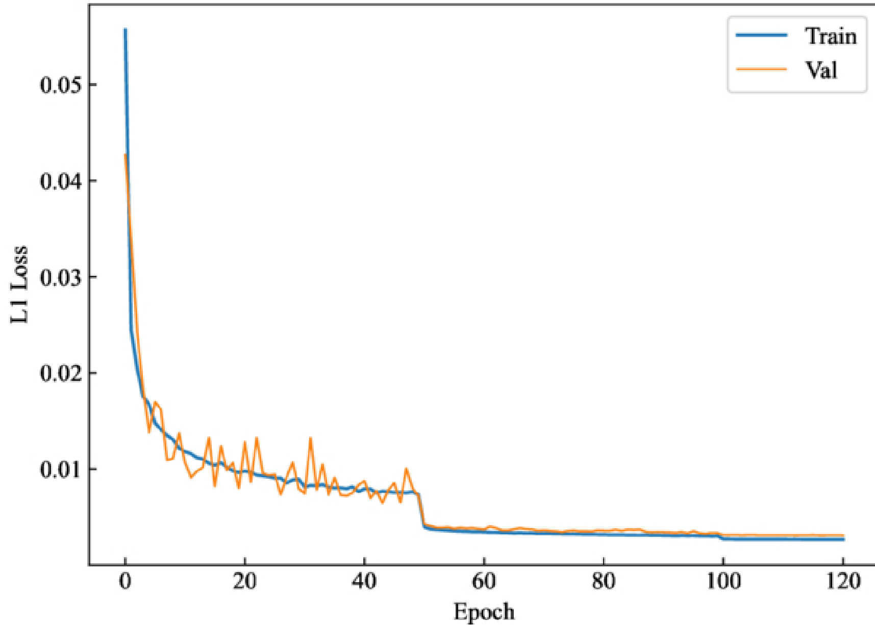
Figure 3. from Jia-Ming Chen et al 2026 Astrophys. J. 1005 doi:10.3847/1538-4357/ae78c7 https://dx.doi.org/10.3847/1538-4357/ae78c7 © 2026. The Author(s). Published by the American Astronomical Society.
