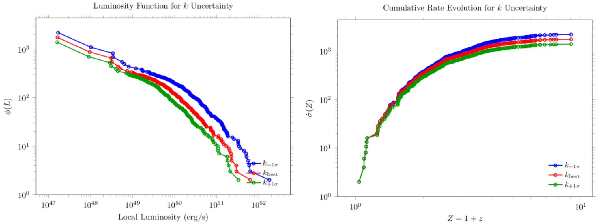
Figure 9. from Sujay Champati et al 2026 Astrophys. J. 1005 doi:10.3847/1538-4357/ae77e2 https://dx.doi.org/10.3847/1538-4357/ae77e2 © 2026. The Author(s). Published by the American Astronomical Society.
