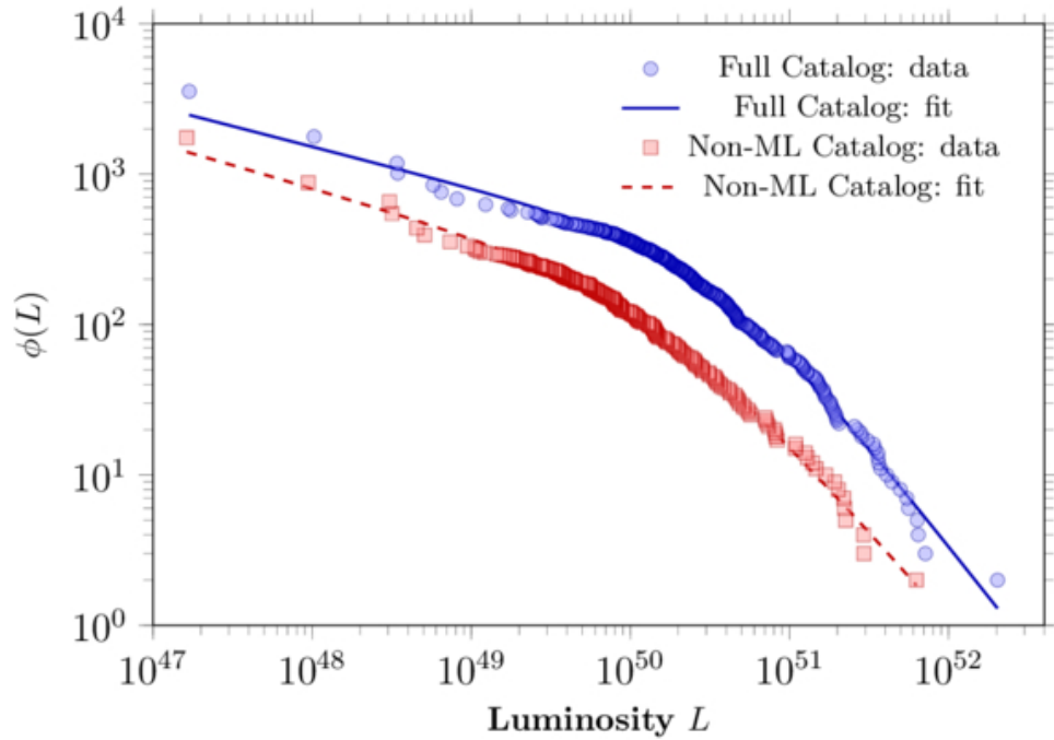
Cumulative Luminosity Functions: Full vs. Non-ML Catalogs
