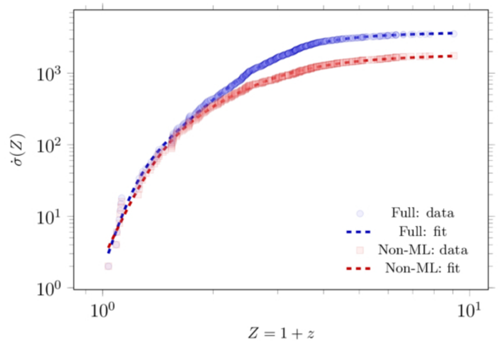
Redshift Evolution: Double-Break Model (Full vs. Non-ML)
