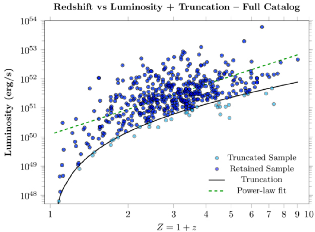
Figure 5. from Sujoy Champati et al 2026 Astrophys. J. 1005 doi:10.3847/1538-4357/ae77e2 https://dx.doi.org/10.3847/1538-4357/ae77e2 © 2026. The Author(s). Published by the American Astronomical Society.
