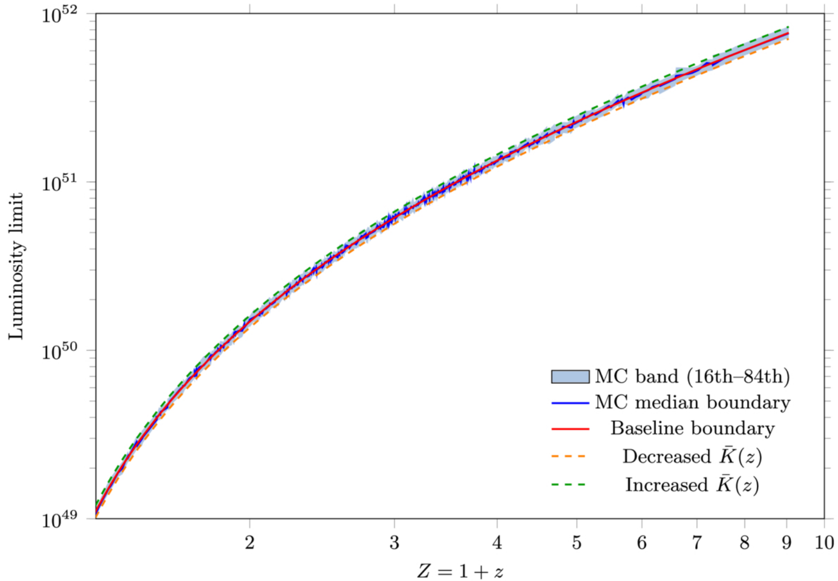
Figure 4. from Sujoy Champati et al 2026 Astrophys. J. 1005 doi:10.3847/1538-4357/ae77e2 https://dx.doi.org/10.3847/1538-4357/ae77e2 © 2026. The Author(s). Published by the American Astronomical Society.
